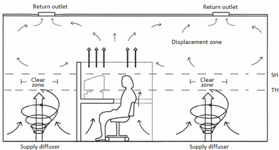
Hybrid Underfloor Air Distribution System
