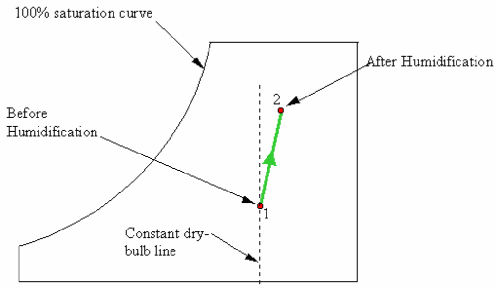
PSYCHROMETRIC CHART SHOWING HUMIDIFICATION
