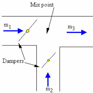
TWO AIR STREAMS MIXING
