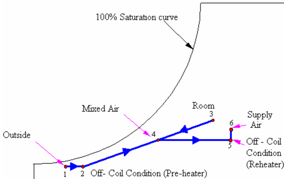
PSYCHROMETRIC CHART SHOWING TYPICAL WINTER CYCLE
