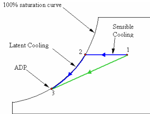
PSYCHROMETRIC CHART SHOWING COOLING AND DEHUMIDIFICATION
