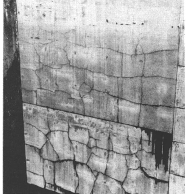
Figure 2-5. Pattern cracking caused by restrained volume changes
