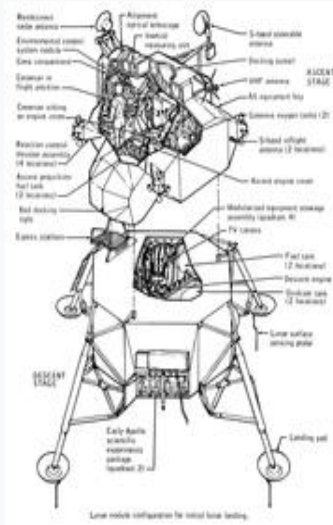
Figure 5. Apollo LM diagram
