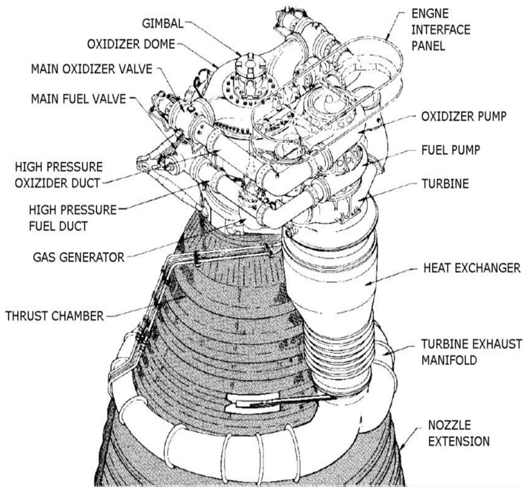
Figure 3. F-1 rocket engine components
