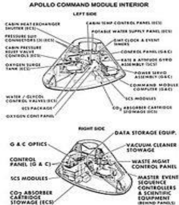
Figure 4. Command module interior arrangement
