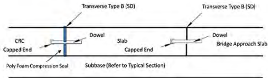
Figure 49. Transition from CRCP using dowelled joints.
