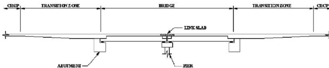
Figure 53. Seamless pavement for transitions of CRCP to and from bridges.
