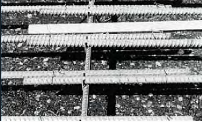
Figure 59. Longitudinal reinforcement lap splices and ties.
