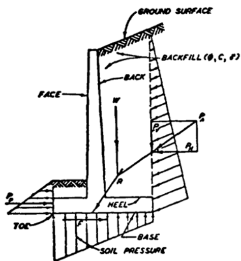
C. CANTILEVER
