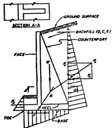
D. COUNTERFORT
