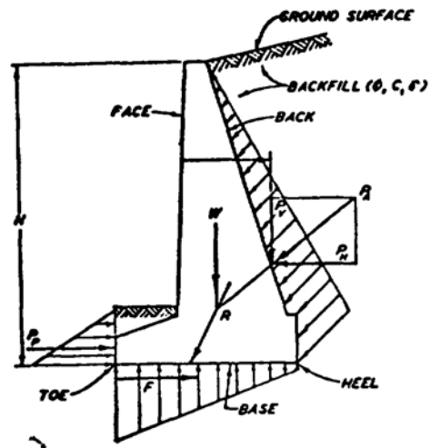
B. SEMIGRAVITY
