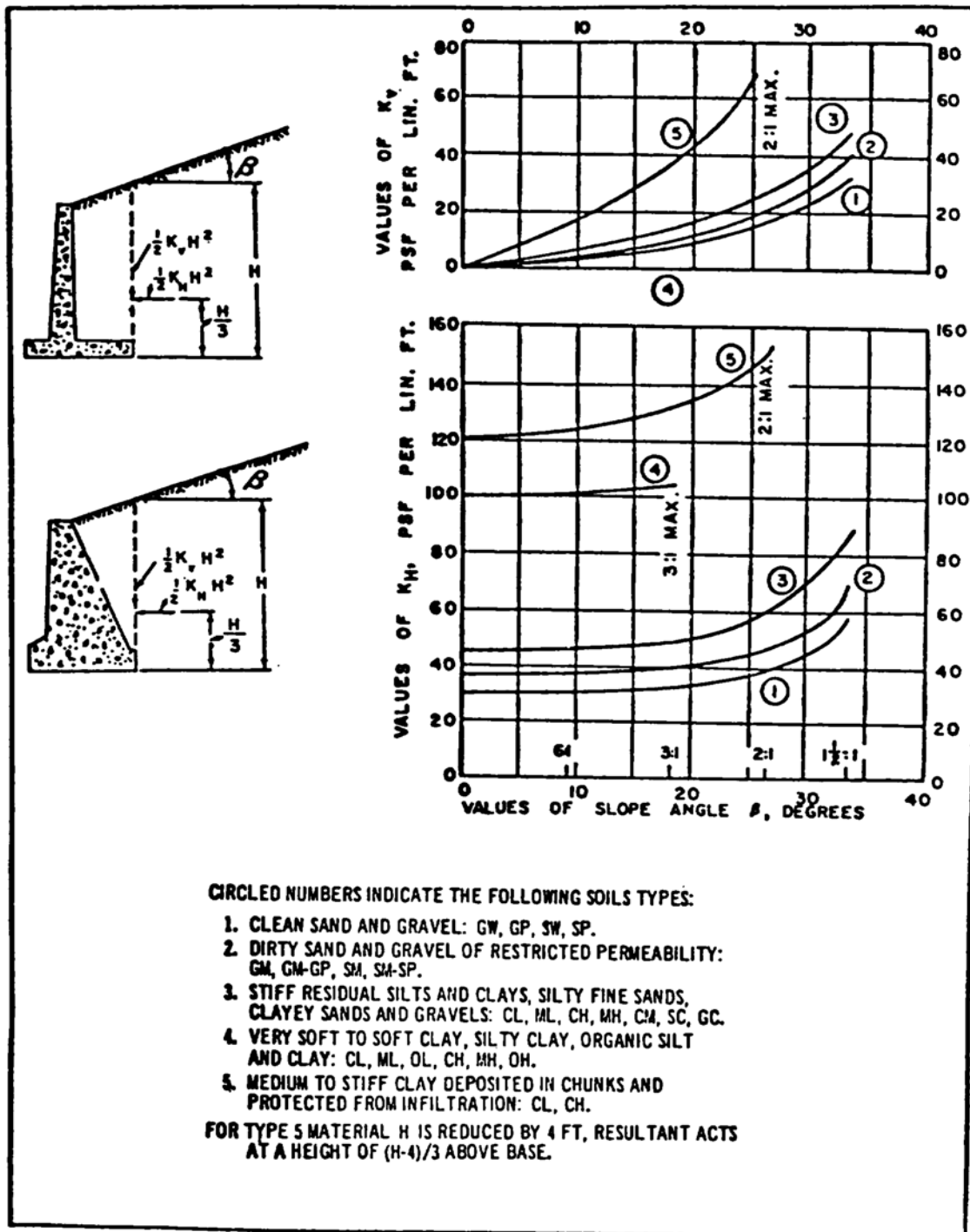
Figure 6 Design loads for low retaining walls, straight slope backfill
