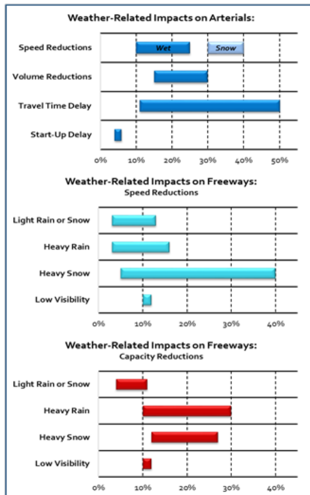
Figure 6. Graph. Weather-Related Impacts on Arterials and Freeways. (Source: Derived from National Highway Traffic Safety Administration historical data)
