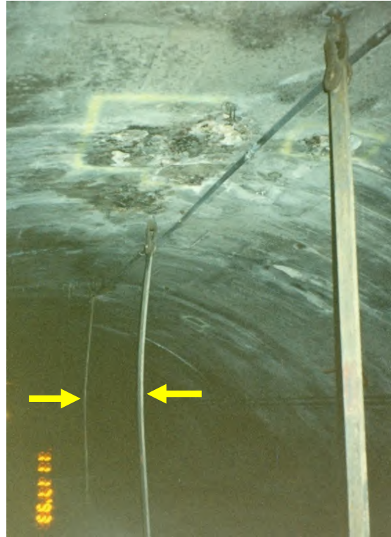
Figure 4.36 – Bent ceiling slab hanger. Note: Successive hangers are bent.
