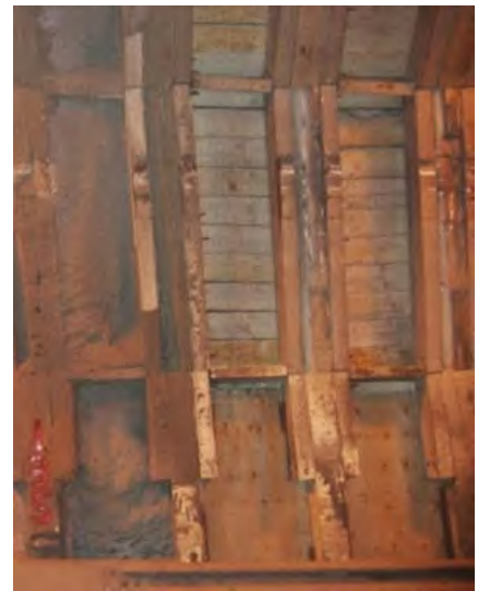
Figure 4.26 – Timber liner in state of deterioration.
