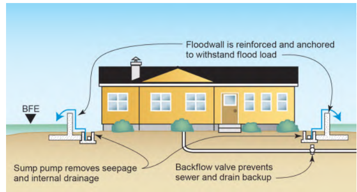
Figure 9: Residential floodwall
