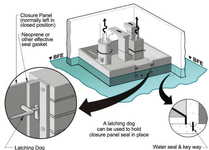
Figure 6: Detail of floodproofed building utility
