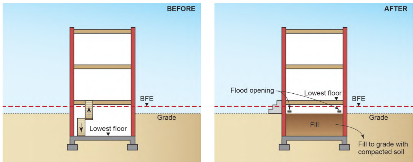
Figure 1: Basement infill before and after mitigation
