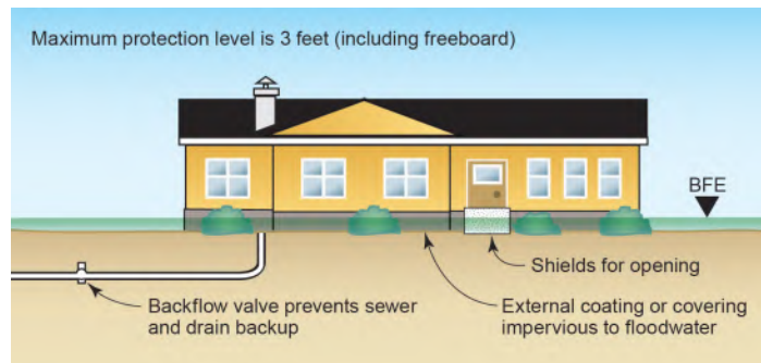
Figure 8: Dry floodproofed building
