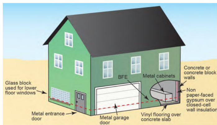
Figure 7: Flood damage-resistant materials
