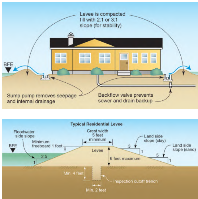
Figure 10: Residential levee and typical levee cross section
