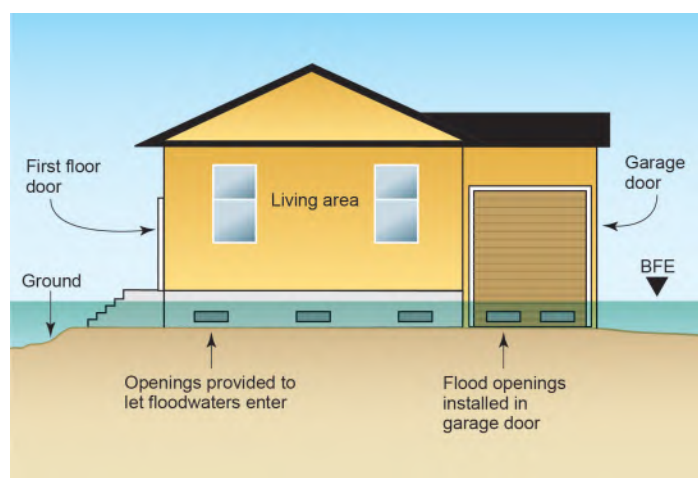
Figure 4: Flood openings and their placement
