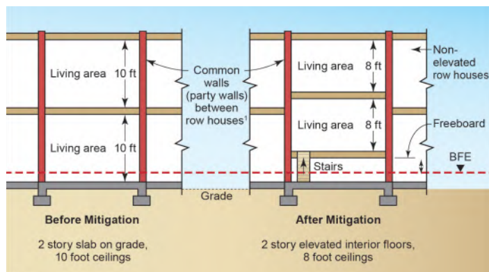
Figure 3: Elevating the lowest interior floor before and after mitigation
