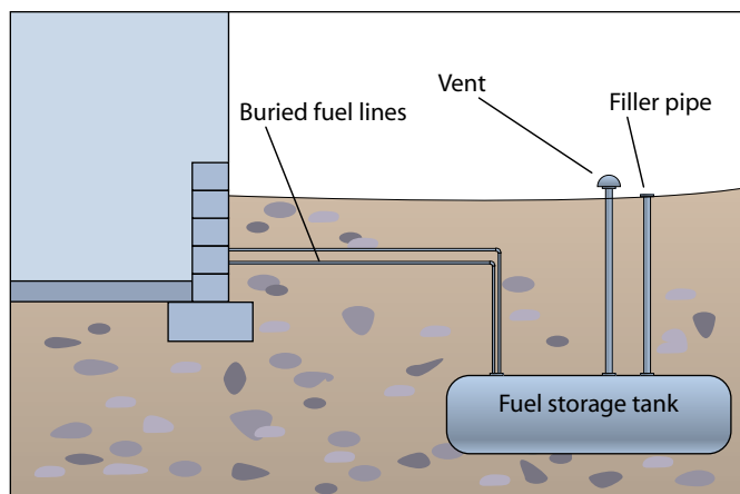
Figure 2. Buried fuel storage tank.
