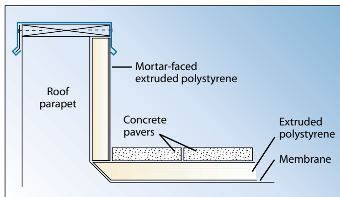
Figure 5. Concrete pavers over membrane (FEMA 55).
