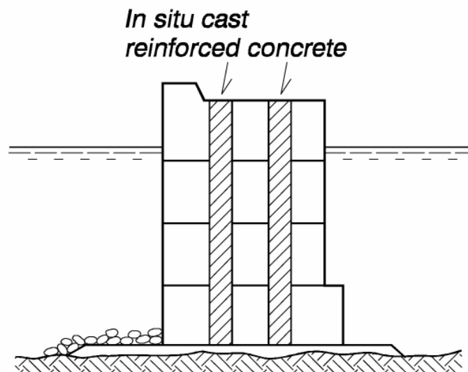
Figure VI-2-21. Example of blockwork breakwater
