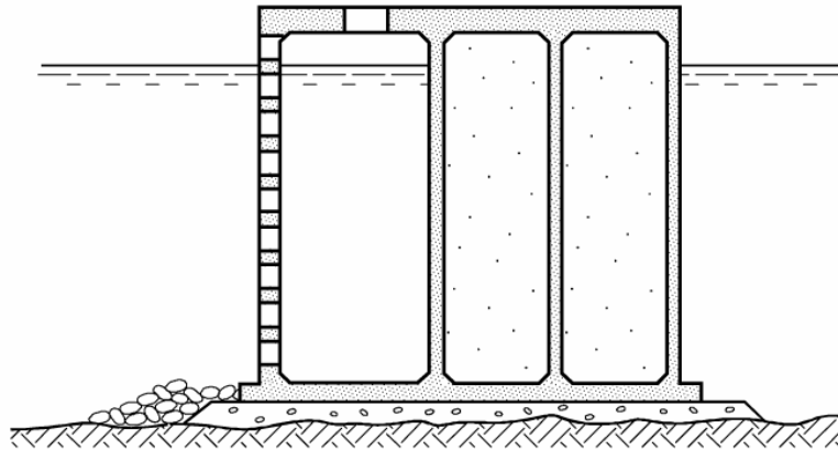
Figure VI-2-20. Perforated front wall caisson breakwater
