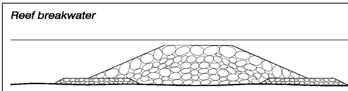
Figure VI-2-15. Example of a reef breakwater
