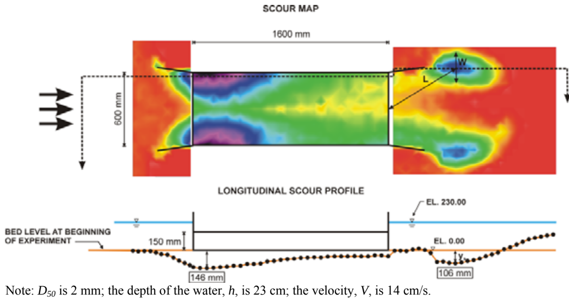
Figure 71. Diagram. Scour map (top) and profile (bottom), submerged with 8-degree wingwalls at outlet and inlet (smooth walls), December 16, 2003.
