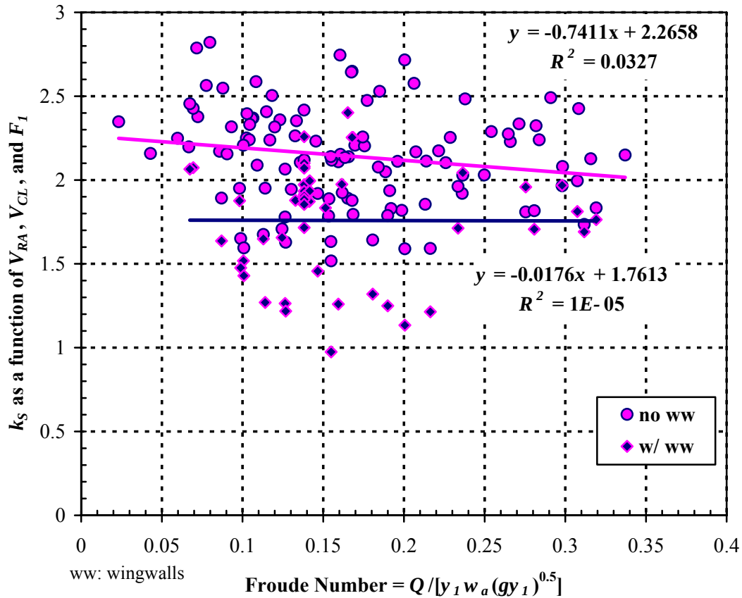
Figure 11. Graph. Calibration of k_S as a function of V_{RA} , V_{CL} , and F_1 .
