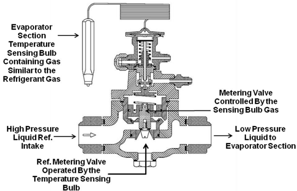
Figure 3.4 Refrigeration System Thermal Expansion Valve
