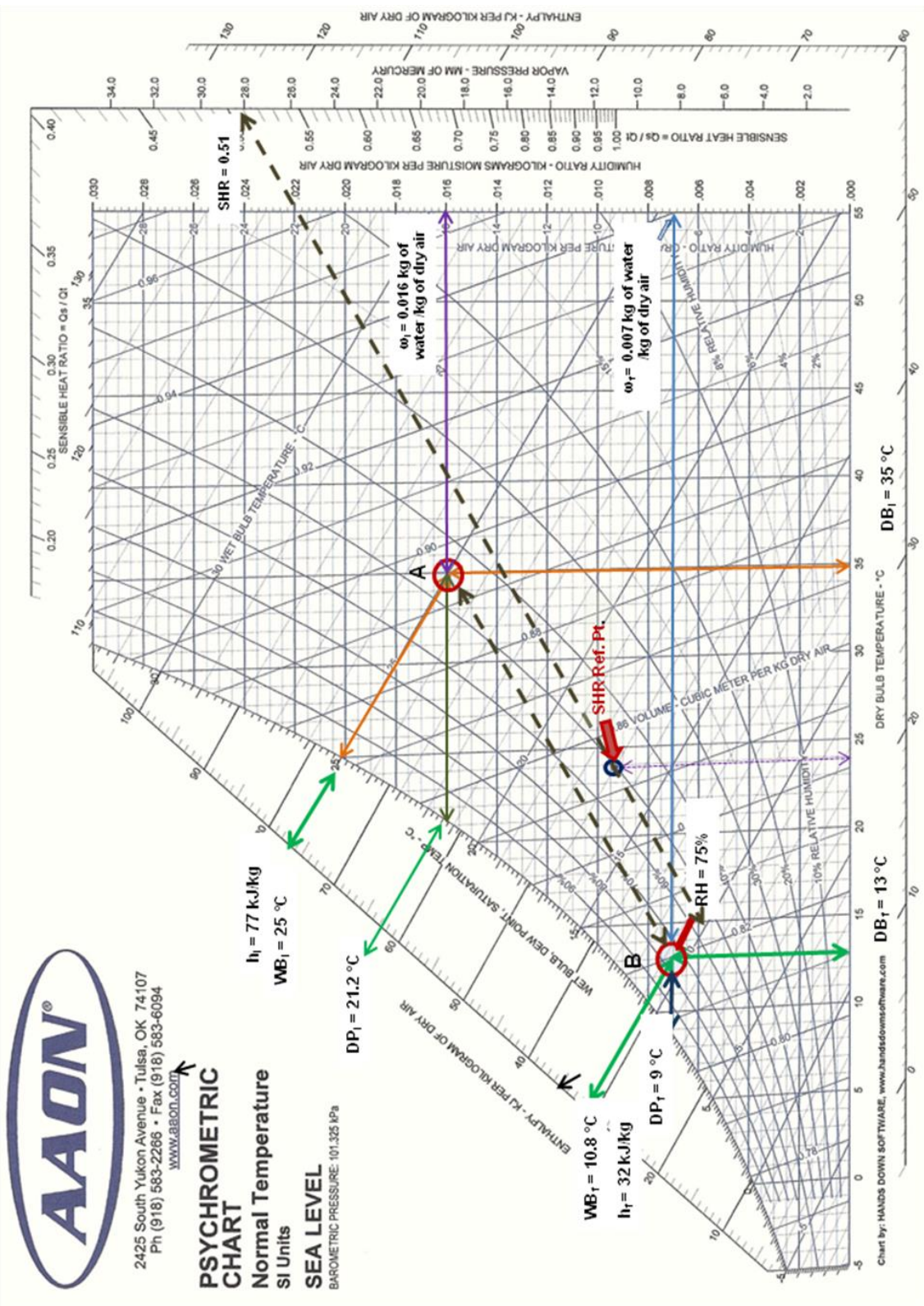
Figure 2.4 Psychrometric Chart – Case Study 2.1, SI Unit System
