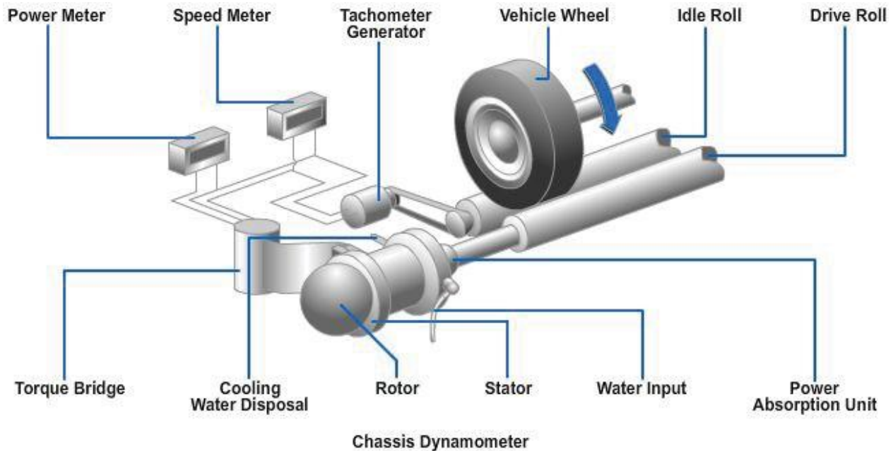
Figure 2-15 – Chassis dynamometer.
