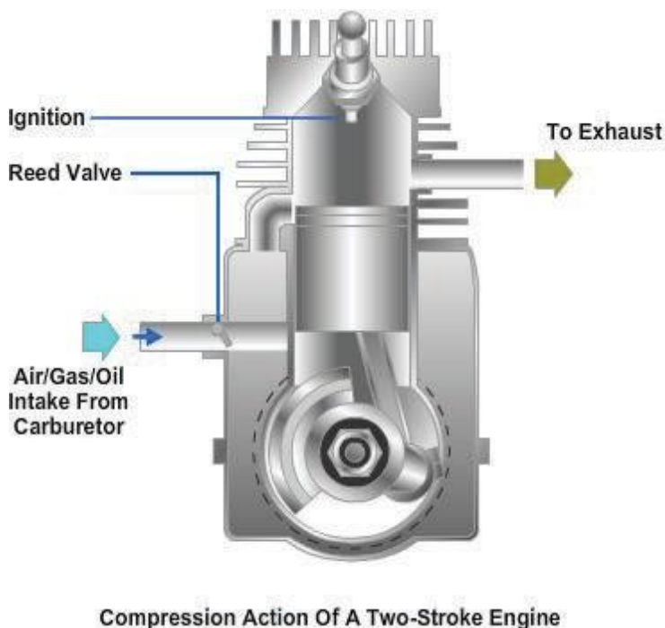
Figure 2-4 – Two-stroke-cycle engine.
