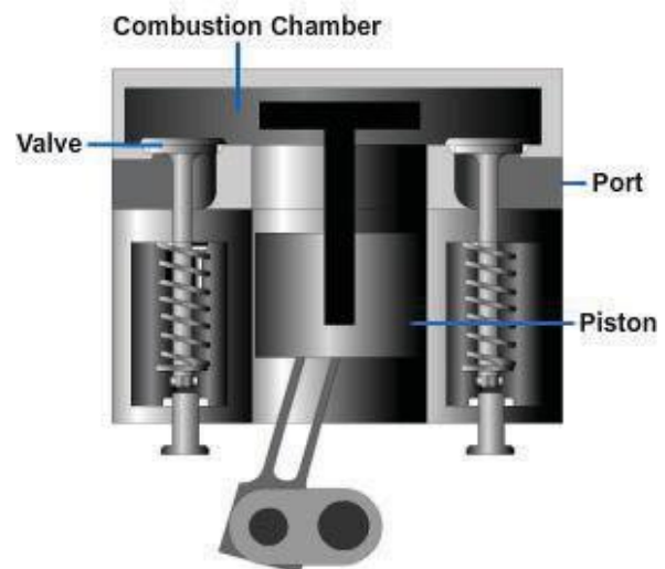
Figure 2-22 - T-Head engine.
