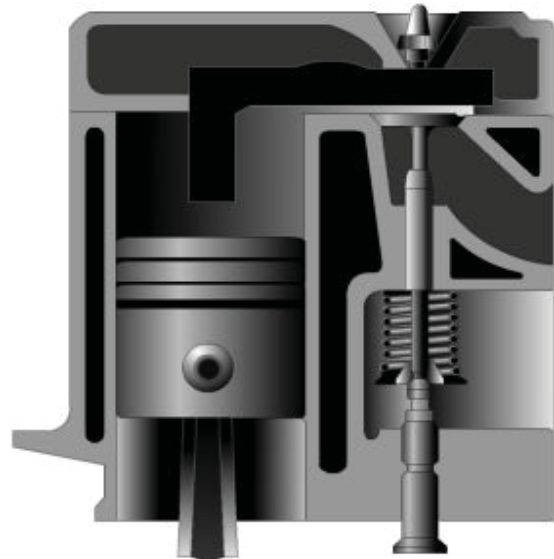
Figure 2-19- L-Head engine.
