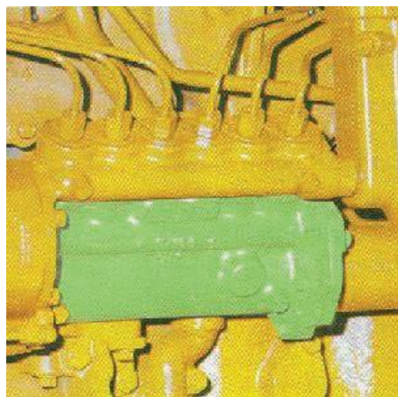
Figure 2-9 - Multiple-plunger, inline pumpsystem.
