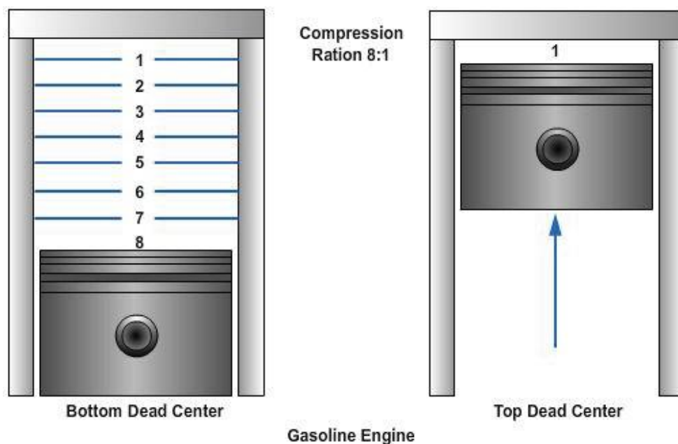
Figure 2-18 – Compression ratio.
