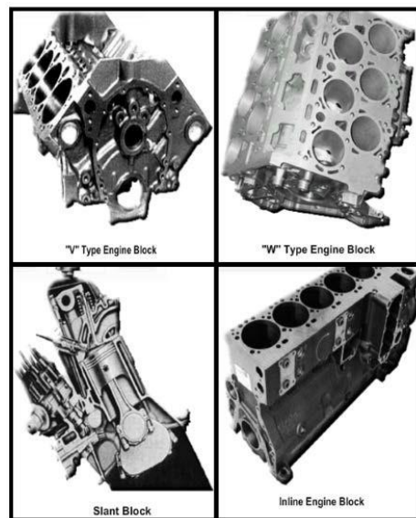
Figure 2-11 - Cylinder arrangements.
