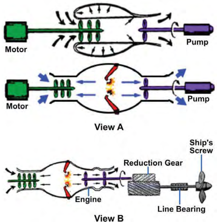
Figure 6-5 — Turbine operating theory.
