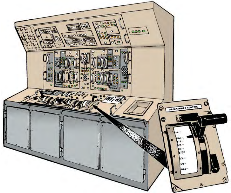
Figure 6-26 — Central control console.
