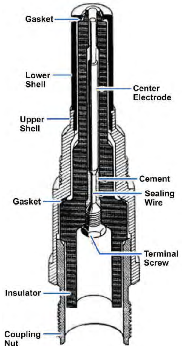
Figure 6-25 — Spark igniter.
