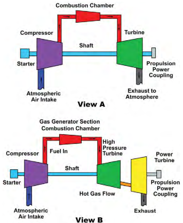
Figure 6-21 — Single-shaft and split-shaft gas turbine.
