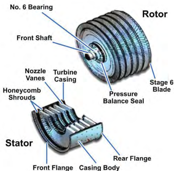
Figure 6-24 — Power turbine.
