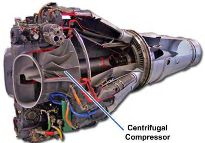
Figure 6-8 — Centrifugal compressor.
