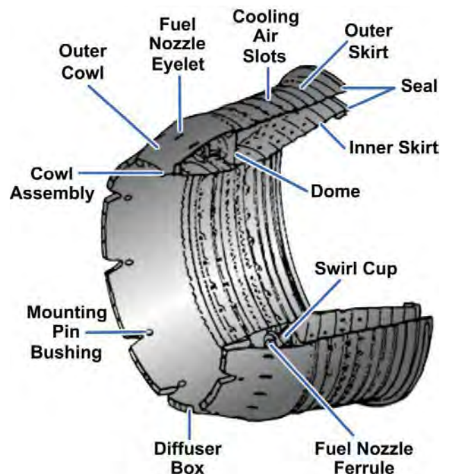
Figure 6-17 — Combustor liner.
