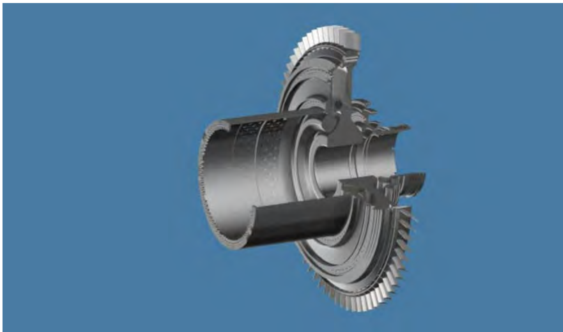
Figure 6-23 — Rotor element of the turbine assembly.
