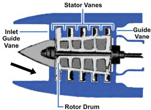
Figure 6-13 — Drum-type compressor rotor.
