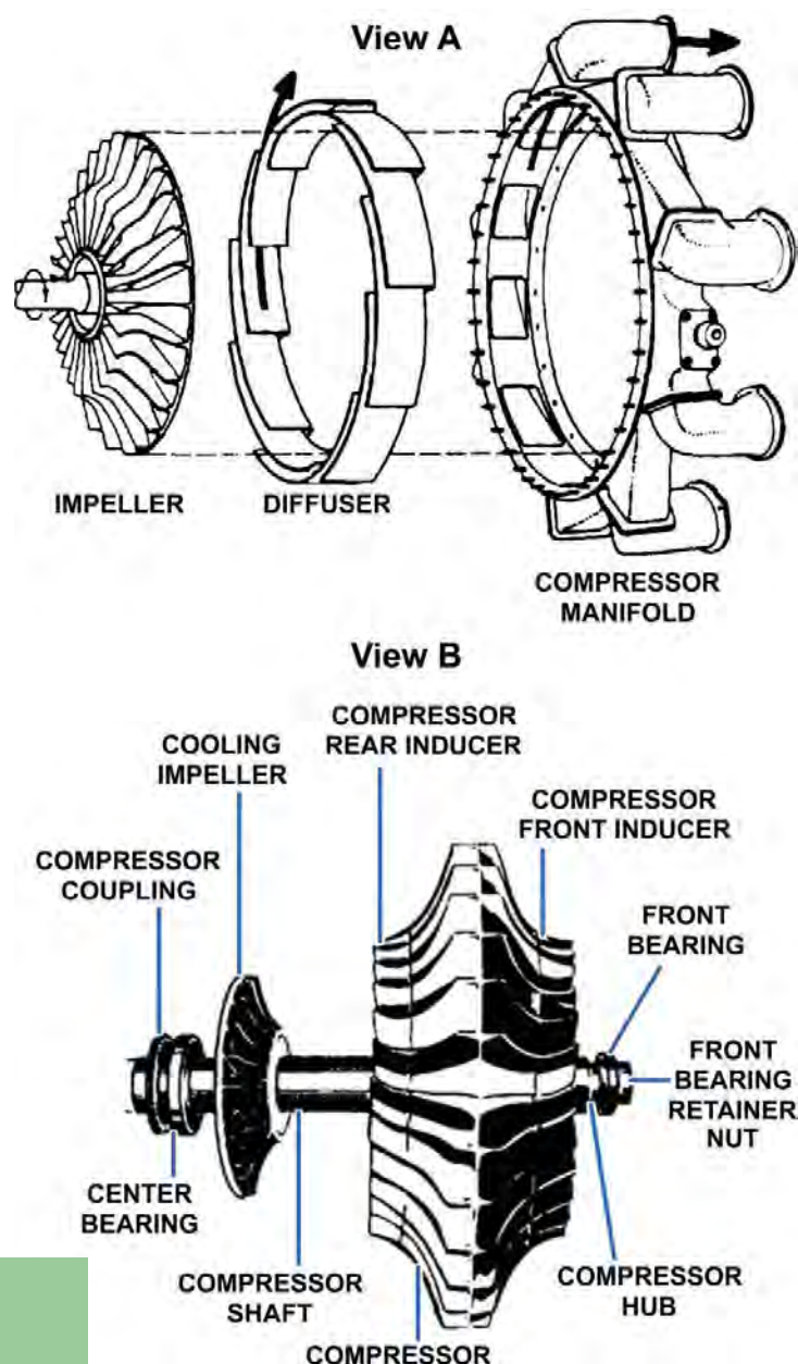
Figure 6-9 — Centrifugal compressor.
