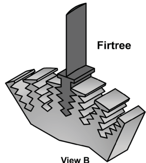
Figure 6-14 — Bulb and firtree root-type rotor blades.
