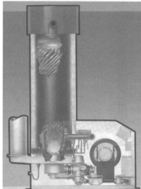
Figure 1. Cutaway View of Water Heater Unit
