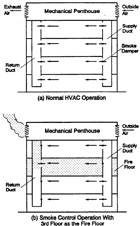
Figure 4. Schematic of Zoned Smoke Control System Using an HVAC System that Serves Many Smoke Control Zones.
