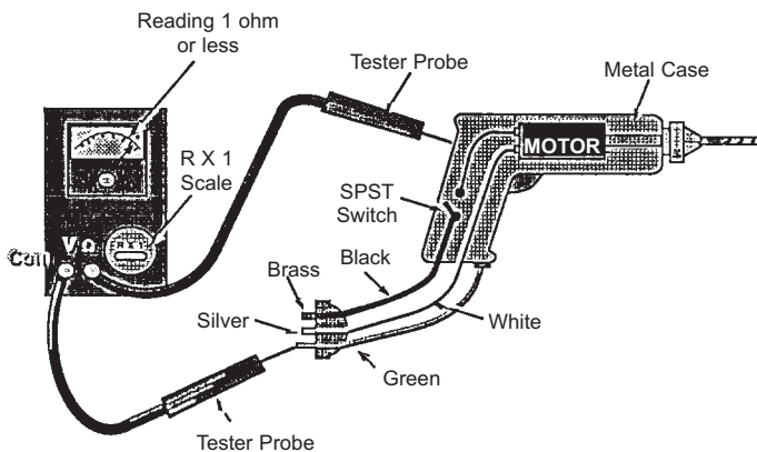
Figure 14 Continuity Test
