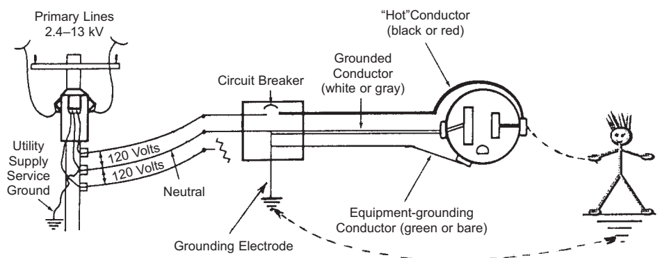
Figure 3 AC Systems—Contact With “Hot” Conductor
