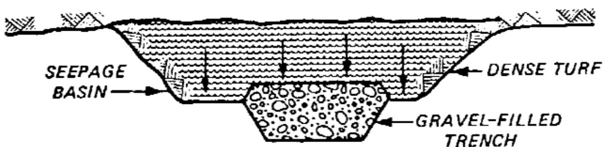
Figure 3-31. Seepage Basin: Shallow Depth to Ground Water
