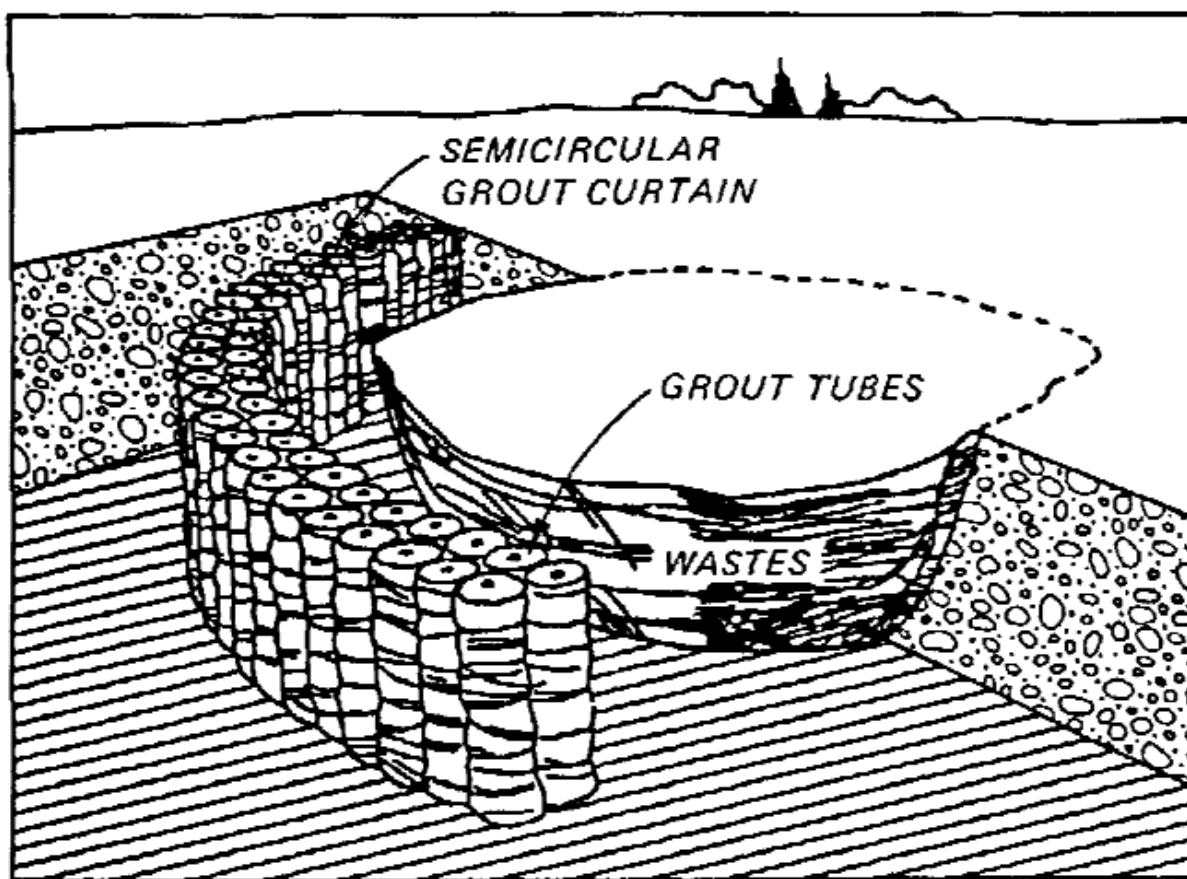
Figure 3-21. Semicircular Grout Curtain Around Waste Site
