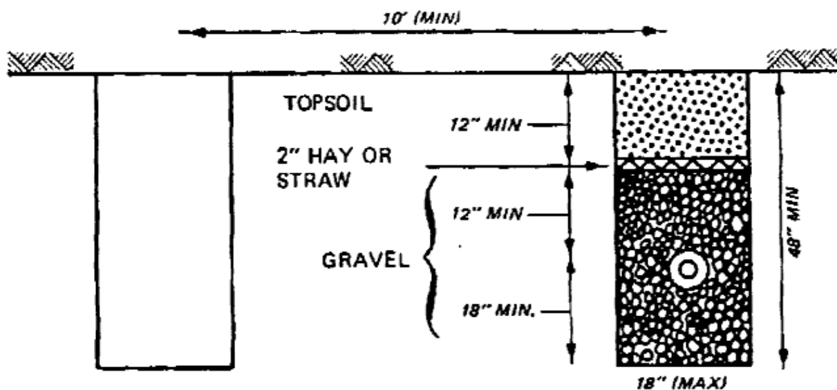
Figure 3-32. Seepage Ditch
