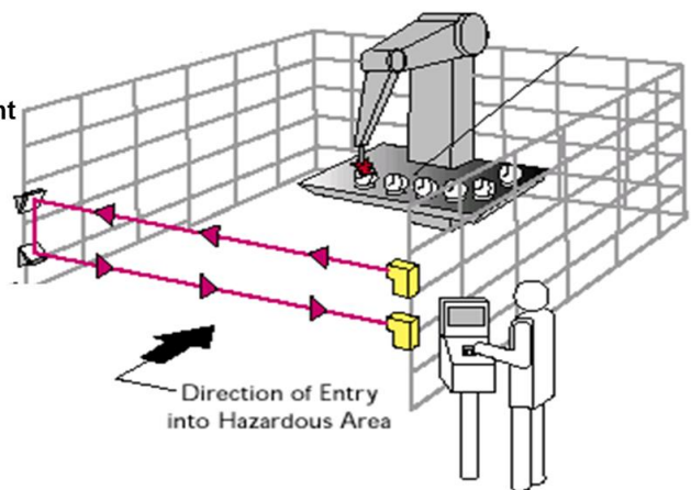
Figure 1.11: Rockwell ® Area Access Control System
