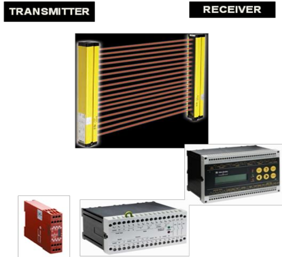
Figure 1.9: Rockwell ® Safety Light Curtain.
