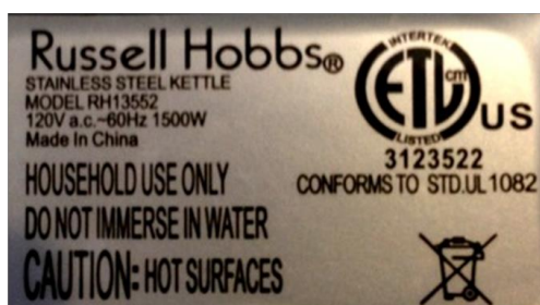
Figure 1.7: Examples of a safety certification labels – ETL and UL Listings.
