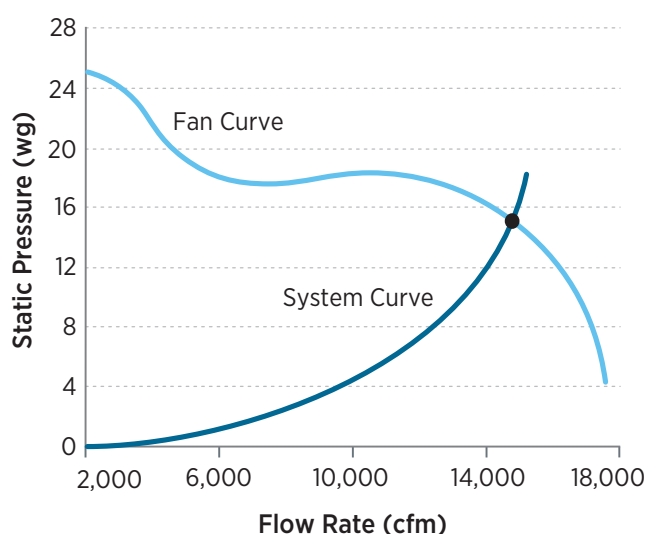
Figure 9. Typical fan and system curves
