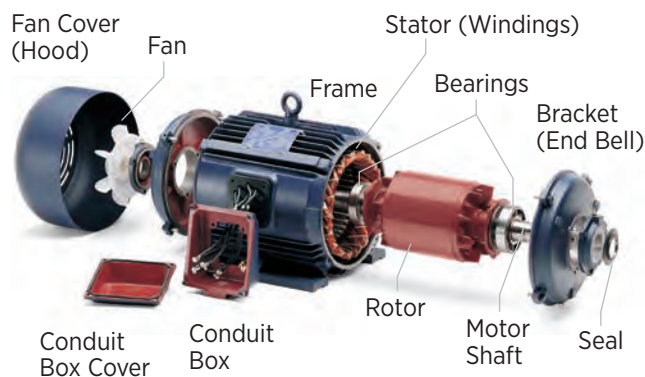
Figure 2. Induction motor Illustration from Leeson Electric Corporation
