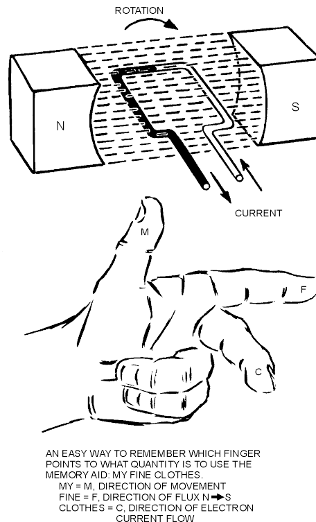
Figure 1-9.—Left-hand rule for generators.
