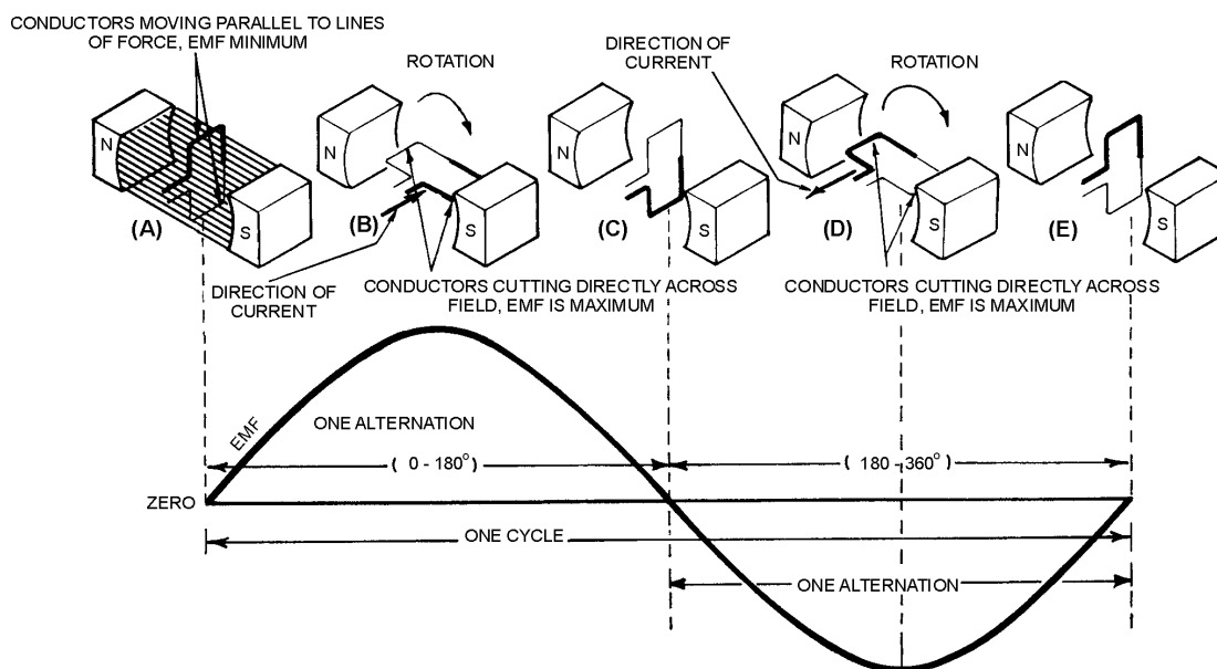
Figure 1-8.—Basic alternating-current generator.
