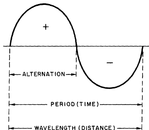
Figure 1-11.—Wavelength.
