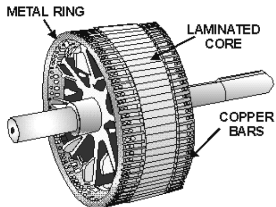
SQUIRREL-CAGE ROTOR
