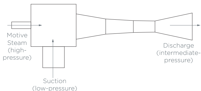
Figure 13. Thermocompressor Operation
