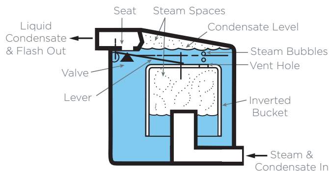
Figure 7. Inverted Bucket Steam Trap
