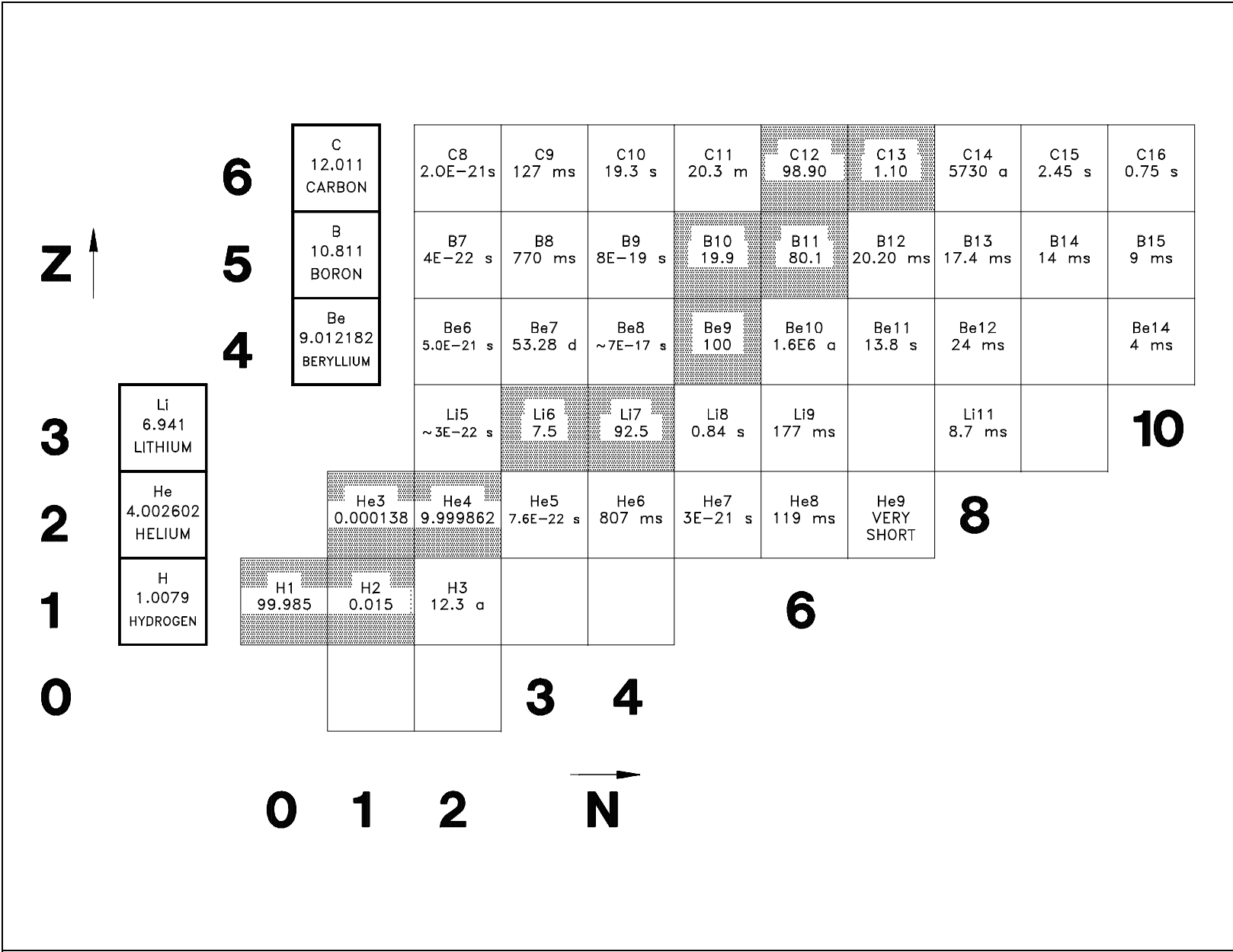
Figure 3 Nucide Chart for Atomic Numbers 1 to 6
