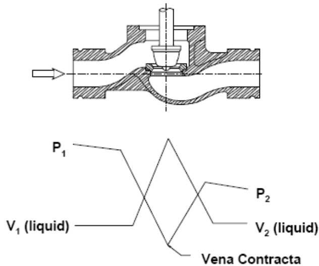
Figure 1.8 Static pressure and velocity profiles across a single seat control valve
