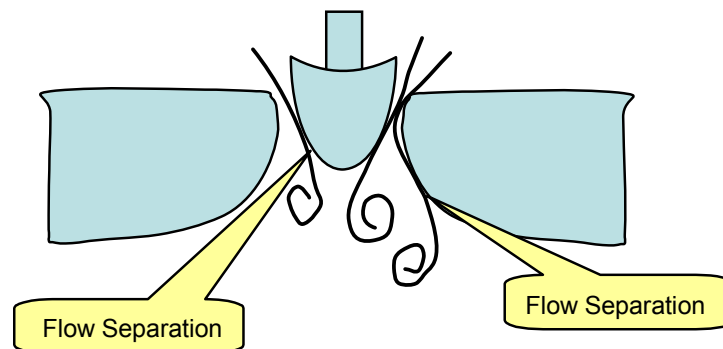
Figure 1.5 Flow separation effects in a single seated globe valve.
