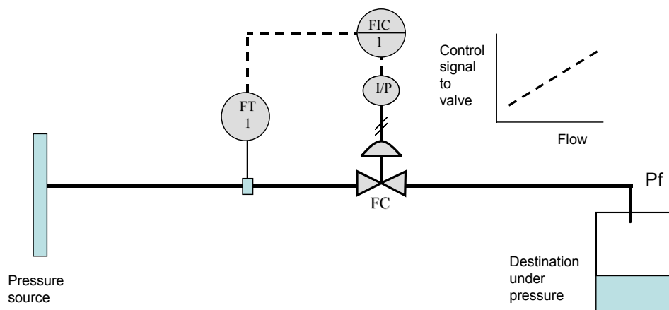
Figure 1.15 Typical flow control arrangement
