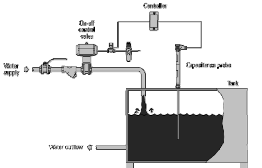
Figure 1.18 An adjustable on/off level control system (Source: International site from Spirax Sarco)
