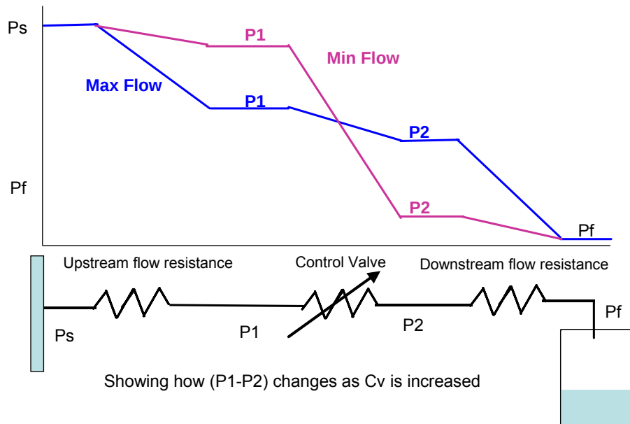
Figure 1.16 Pressure profile for gas at critical flow through a single seat globe valve
