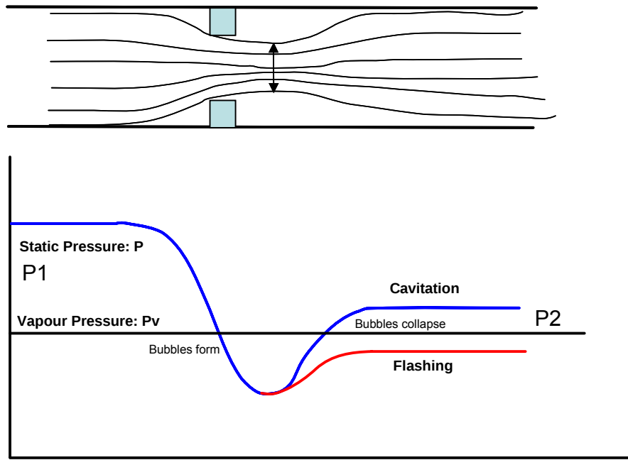
Figure 1.11 Pressure profiles for flashing and cavitation
