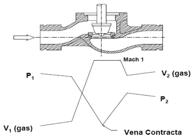
Figure 1.14 Pressure profile for gas at critical flow through a single seat globe valve
