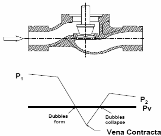
Figure 1.12 Pressure profile for cavitation in a single seated globe valve
