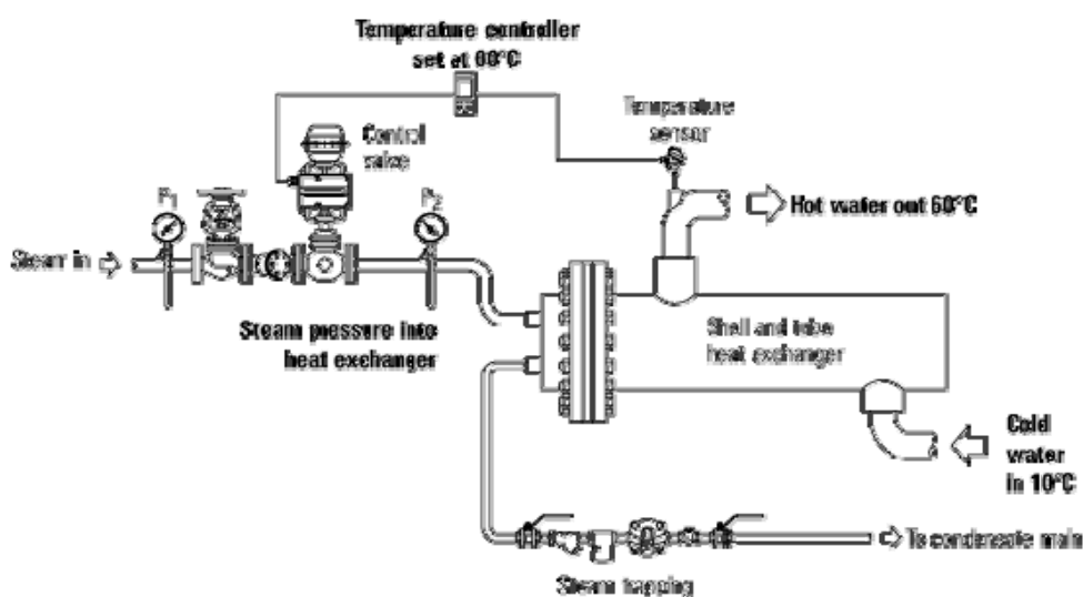
Figure 1.17 Typical temperature control of a steam/water shell and tube heat exchanger (Source: International site from Spirax Sarco)
