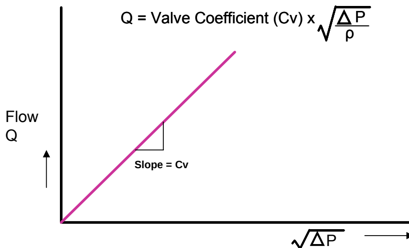
Figure 1.9 Basic flow versus pressure drop relationship for a control valve (sub-critical flow)
