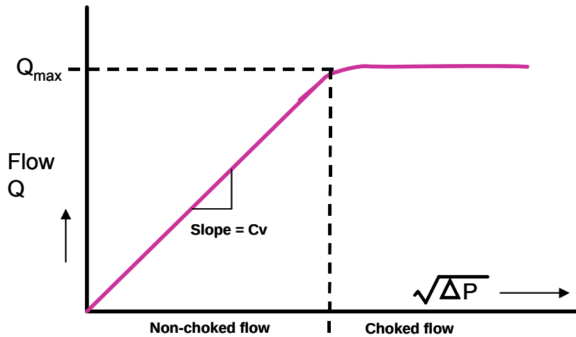
Figure 1.10 Flow versus DP for liquid control valve showing choked flow.
