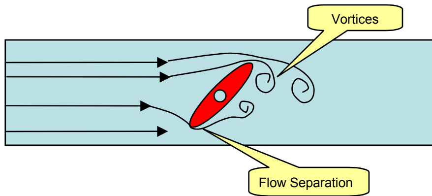
Figure 1.4 Flow separation effects in a butterfly valve.
