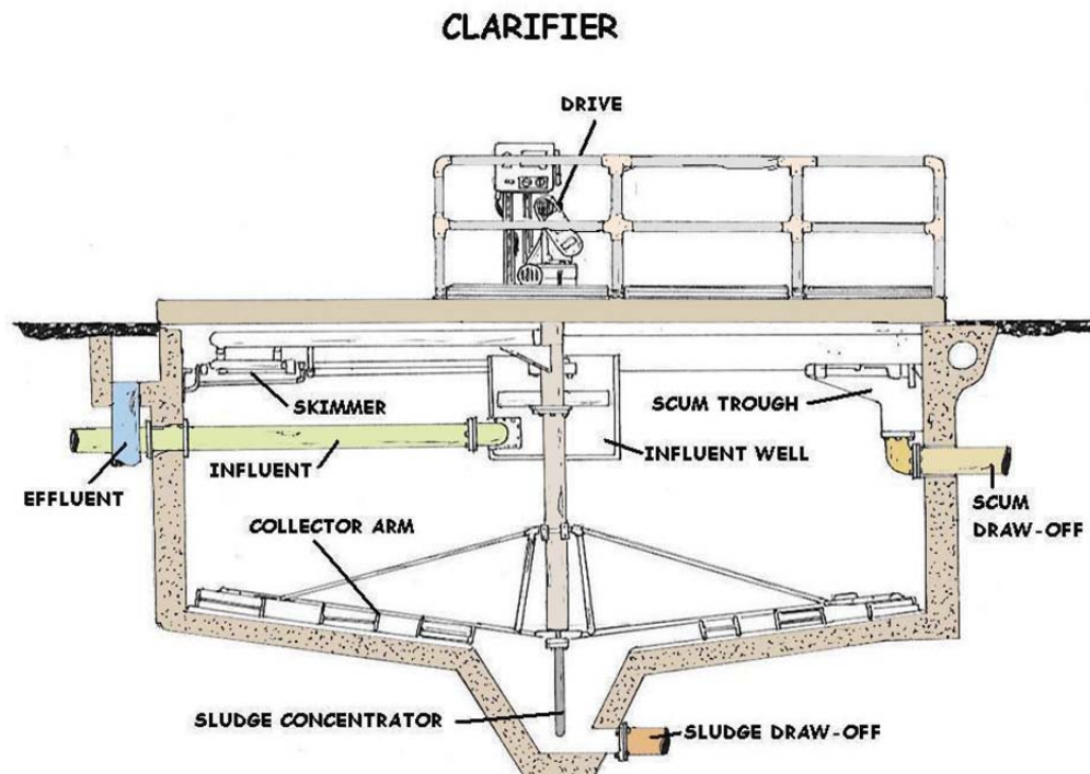
Circular clarifier and collector mechanism.
