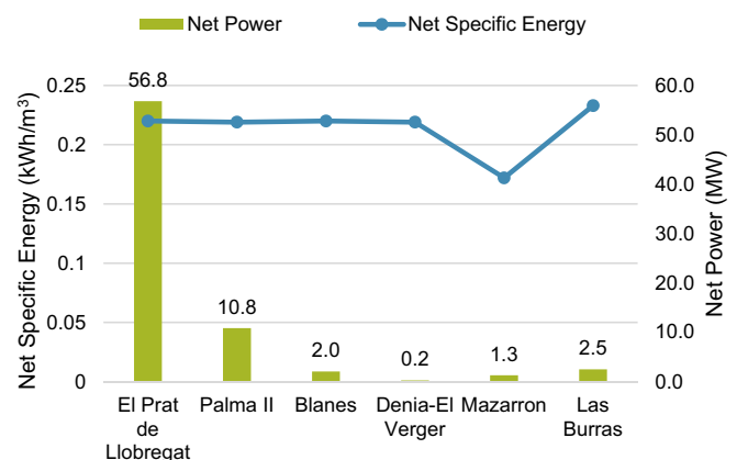
Fig. 4. Simulated net power and specific energy obtained in specific scenarios.
