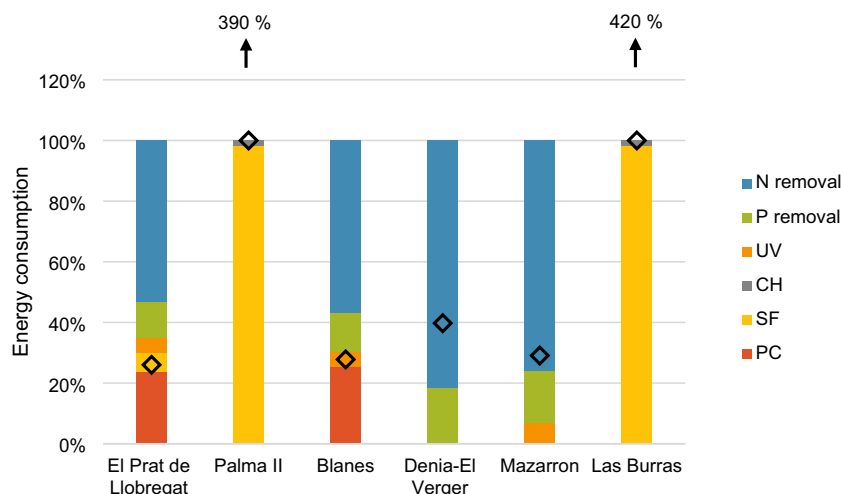
Fig. 5. Distribution of tertiary treatment energy by type of treatment and percentage of energy covered by SGE (◆).
