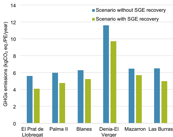
Fig. 6. Estimated carbon dioxide emissions present and in the future by implementing SGE energy recovery.
