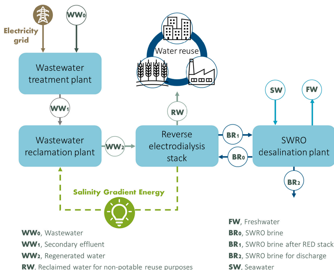
Fig. 1. Outline of the planned water reclamation and brine waste energy valorisation.
