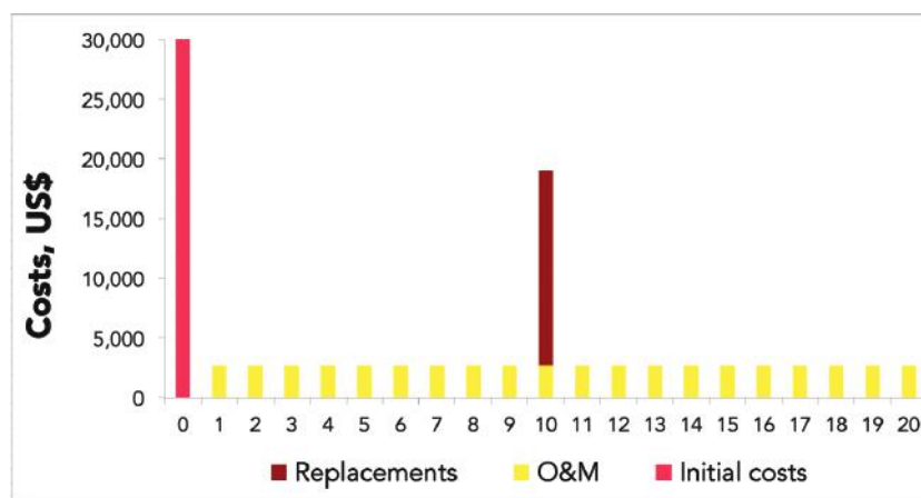
Figure 6. Yearly costs of a hypothetical solar pumping system.
