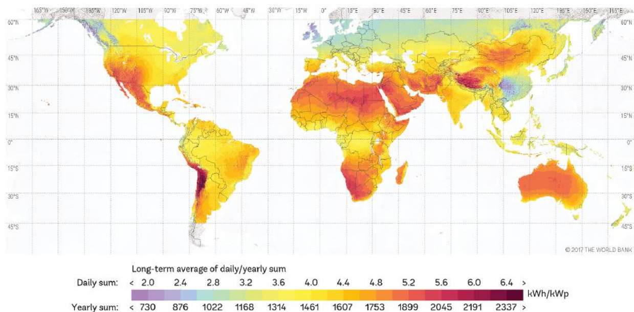
Figure 3. Global solar radiation map. Source: The World Bank.
