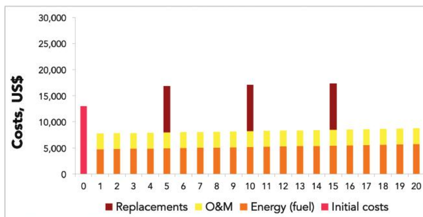
Figure 5. Yearly costs of a diesel-based pumping system.
