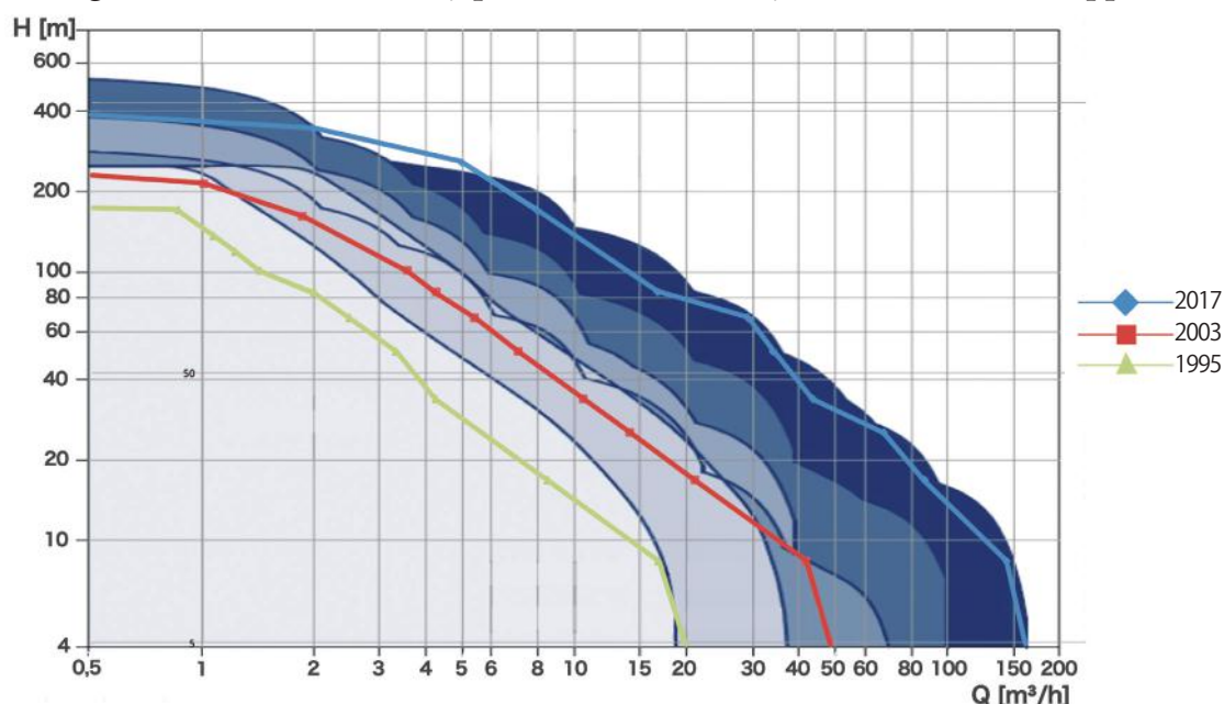
Figure 1. Solar pump capacity has increased due to technology innovations. Image credit: Grundfos.
