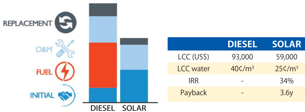
Figure 7. Economic comparison of diesel with solar pumping.
