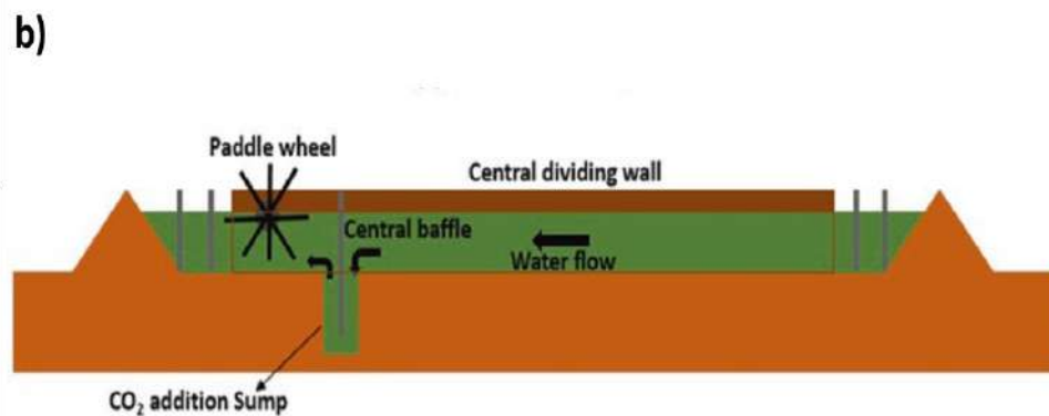
Figure 4.2.8: Schematic diagram of high rate algal ponds a) Paddle wheel in HRAP b) Side elevation view of HRAP (Source: Ranjan et al., 2019)
