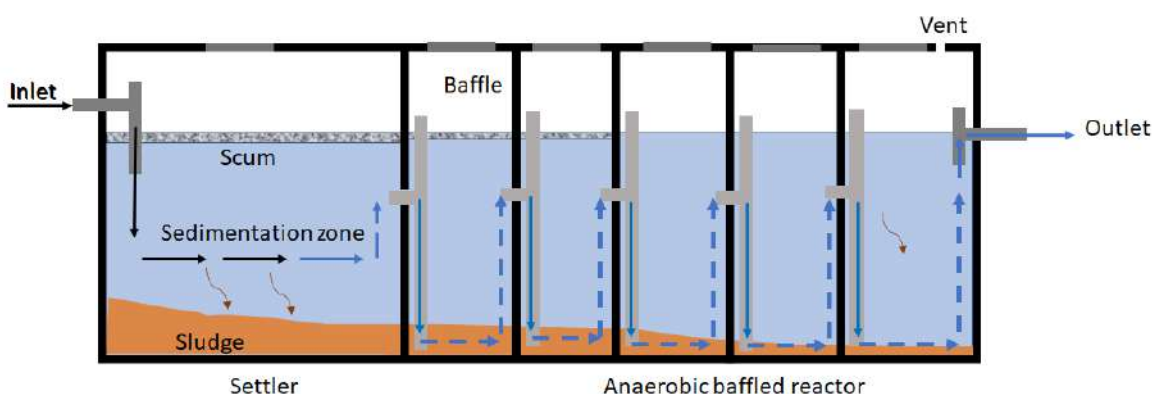
Figure 4.3.4. Anaerobic Baffled Reactor septic tank showing location of baffles and three distinct layers (scum (oil, fats, and grease), clarified water, and sludge (Source: Tilley et al., 2014)
