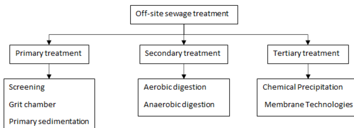
Figure 3.3.2 : Primary, secondary, and tertiary treatment methods of an off-site wastewater treatment system
