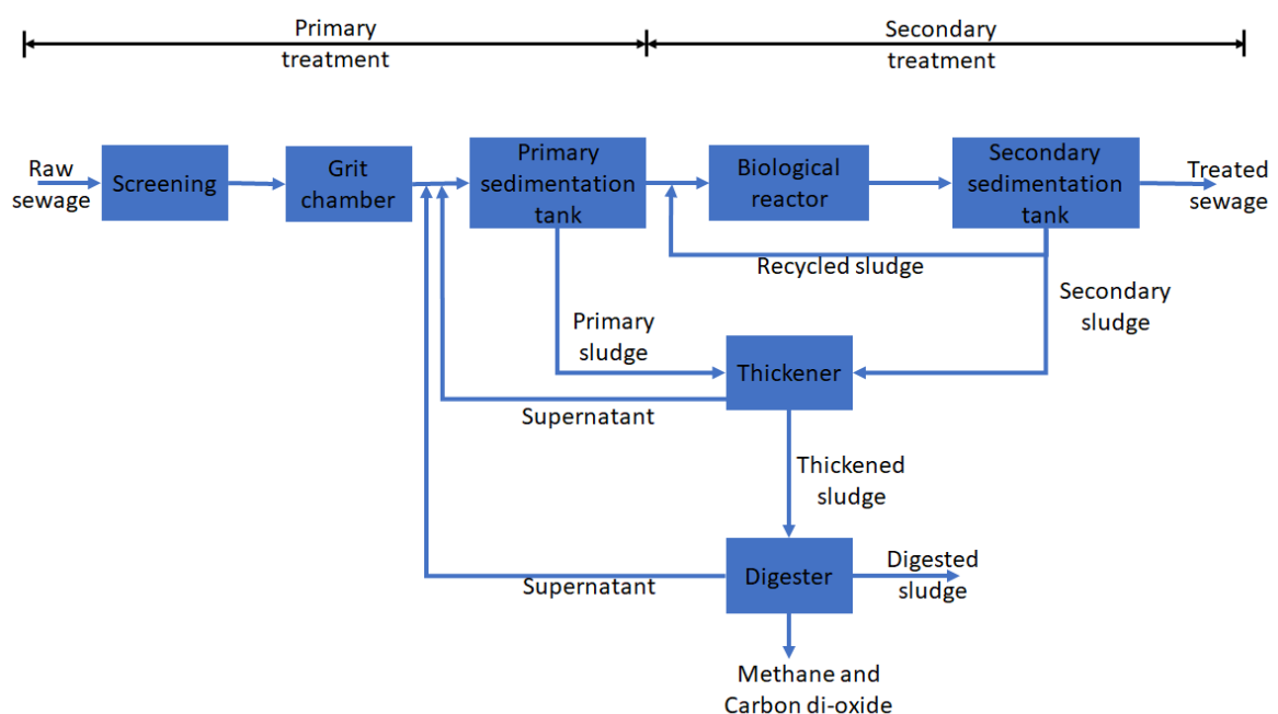
Figure 3.3.4 : Sewage flow through the primary and secondary treatment units of an STP (Source: CPCB, 2013)
