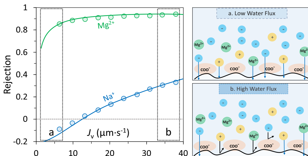
Fig. 4. Ion rejection by NF membranes from solution with monovalent and divalent cations as function of permeate flux, J_v . Lines are theory and symbols are experimental data from Déon et al. ( [\text{Cl}^-]_{\text{tot}} = 100 \text{ mM} ). Model parameters in Table 2, Case II [40].
