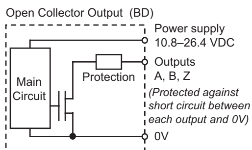
Image 4: Open Collector
