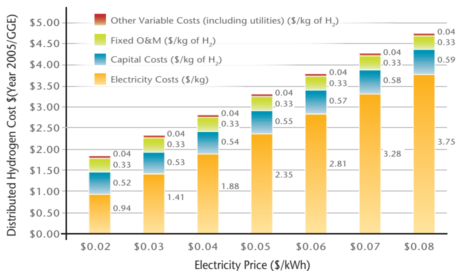
Figure 3. Effect of Electricity Price on Distributed Hydrogen Production Cost (assumes 1,500 GGE/day, electrolyzer system at 76% efficiency, capital cost of $250/kW)
