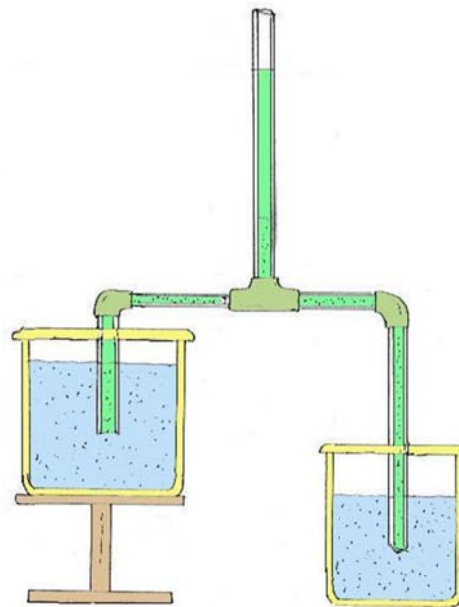
PASCAL'S SIPHON
