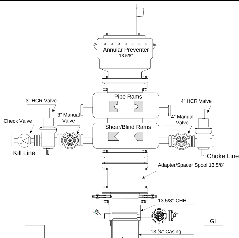
Figure 2-33: Class (III) & (IV) BOP Stuck
