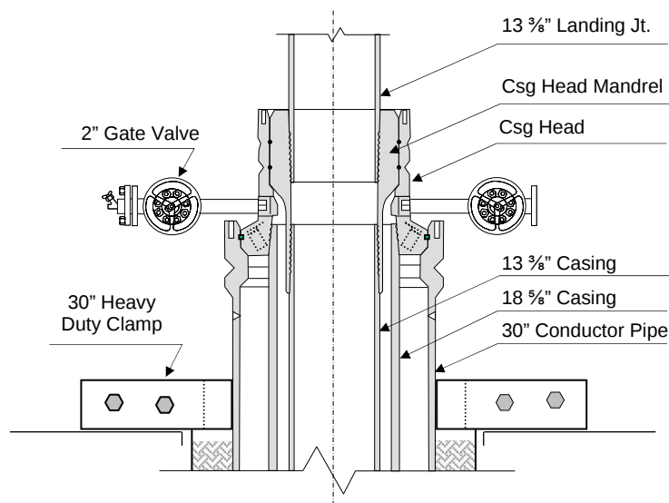
Figure 2-26: 13 ⅜" Casing landed on CH Mandrel
