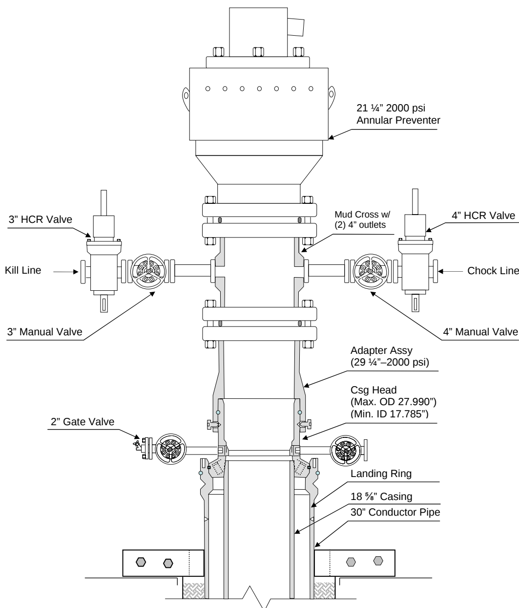
Figure 2-21: BOP Stack for Drilling 17.1/2" Hole
