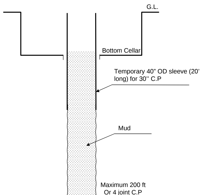
Figure 2-1: Running temporary sleeve & drilling hole prior to run C.P with piling machine
