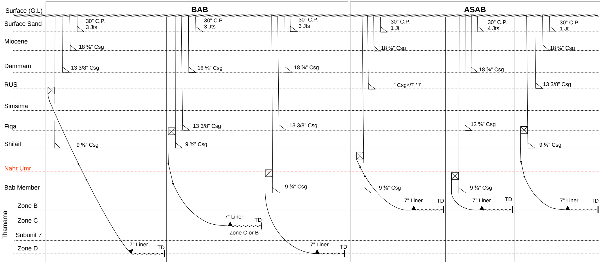
Figure 2-38: ADCO's Typical 6" Hole
