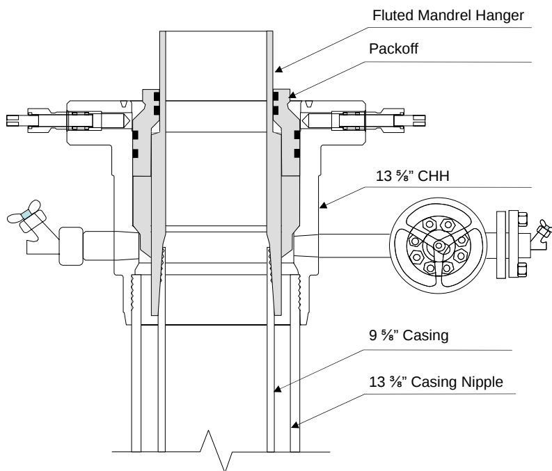
Figure 2-36: 9 5/8" casing landed on CHH with Fluted Mandrel Hanger after cementing
