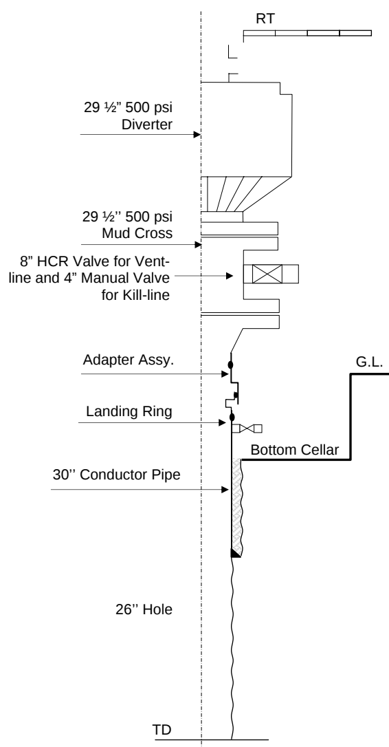
Figure 2-16 : Drilling 26" Hole through 29 1/2" Diverter
