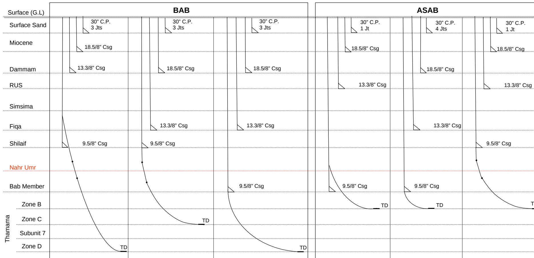
Figure 2-37: ADCO's Typical 8 1/2" Phase
