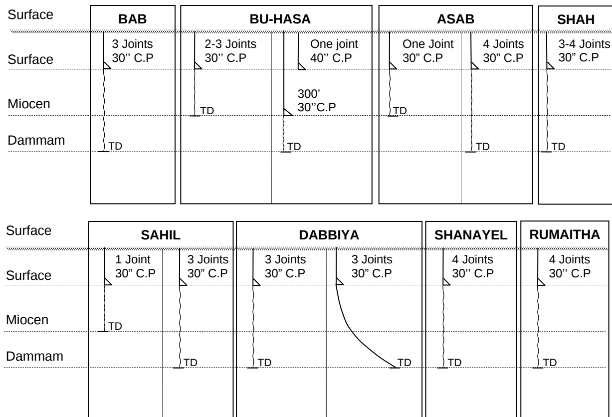
Figure 2-14: ADCO's Typical 26" Phase
