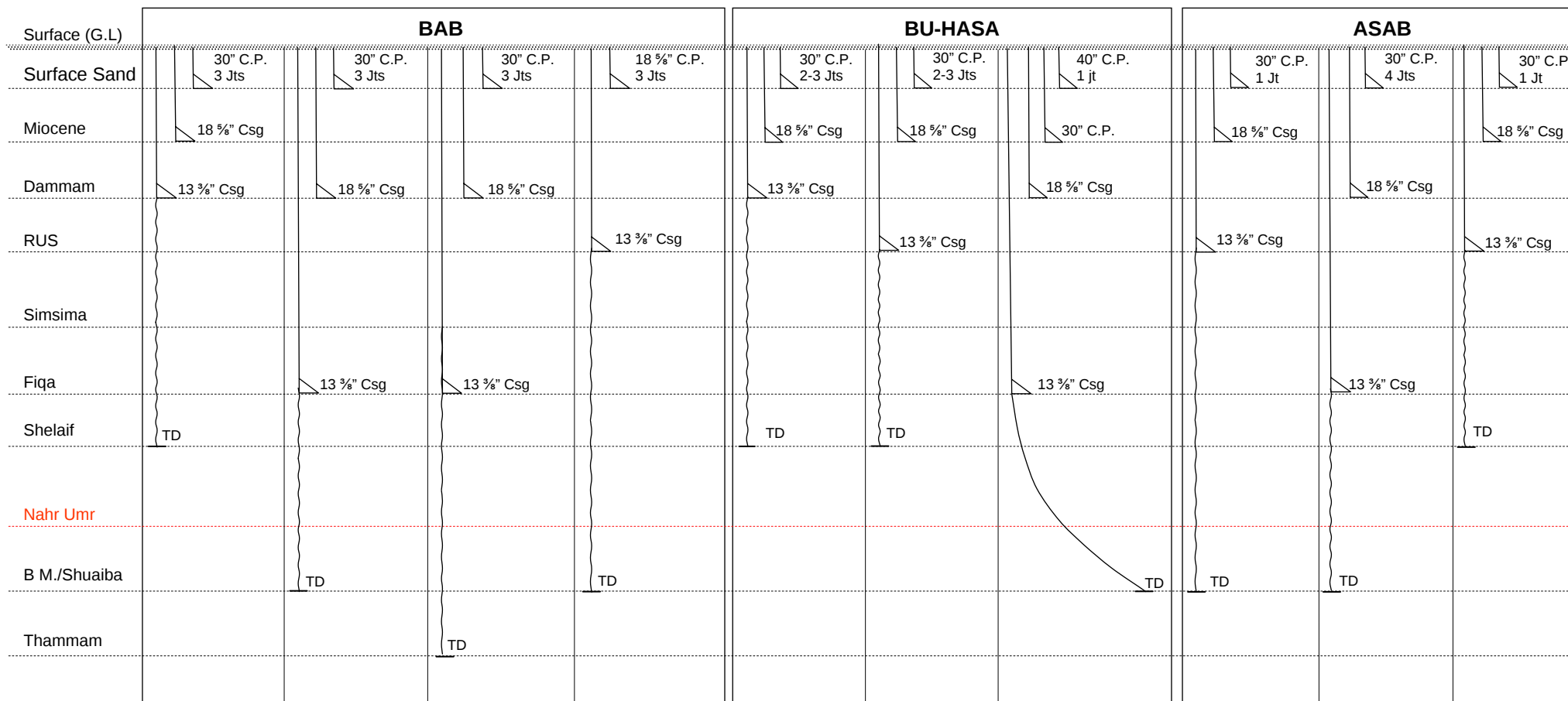
Figure 2-34: ADCO's Typical 12 1/4" Phase
