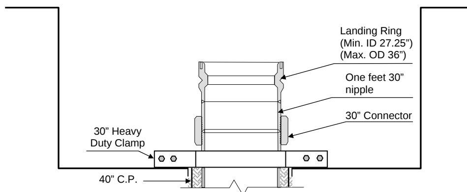
Figure 2-11: landing ring and one ft nipple made up to the C.P prior to cementing
