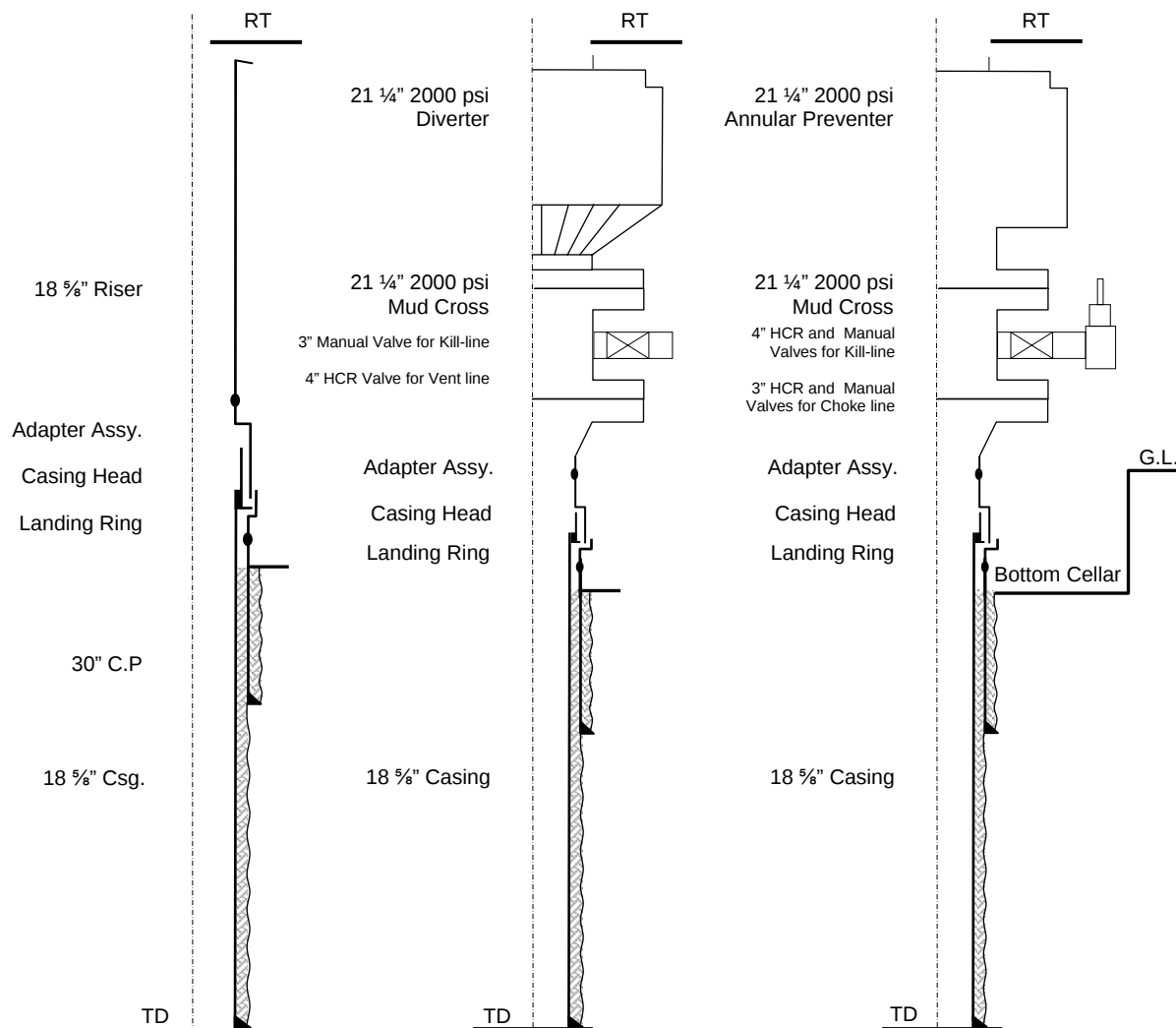
Figure 2-25: Drilling 17 1/2" Hole through 21 1/4"x2000 psi Annular preventer
