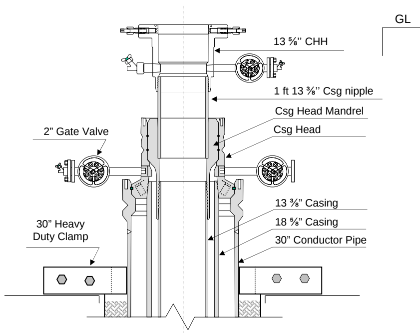
Figure 2-30: 13.5/8" Thread Type CHH after landing 13 3/8" casing
