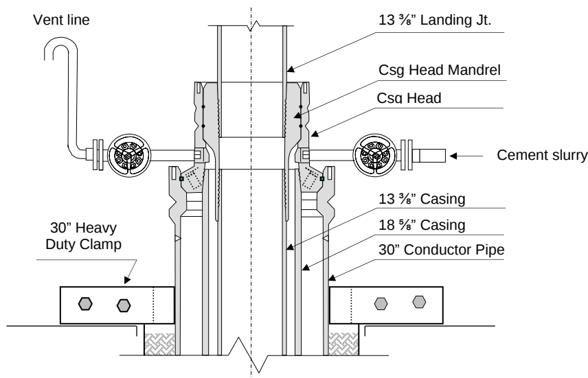
Figure 2-28: Top job of 13 3/8" Casing in case of empty annulus
