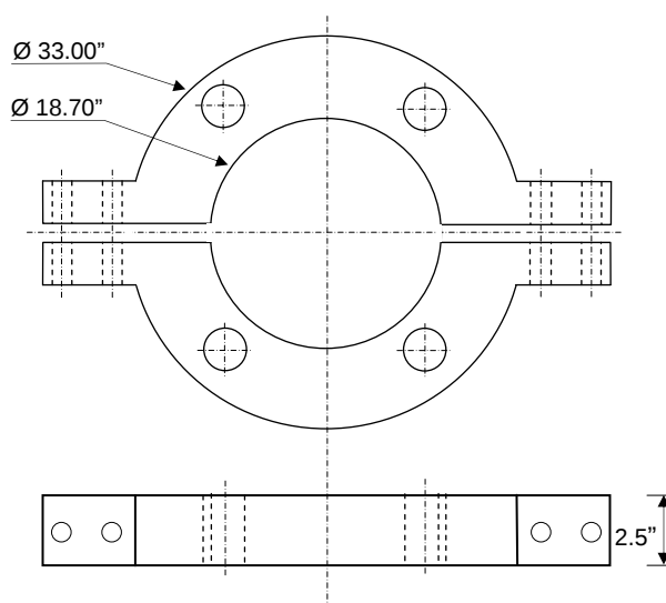
Figure 2- 17:- Heavy Duty Clamp for Landing 18 5/8" Casing
