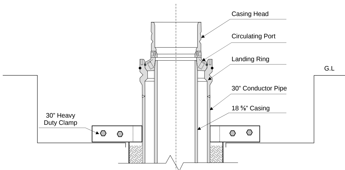
Figure 2-19: Mud Riser or Diverter removed after landing 18 5/8" Csg
