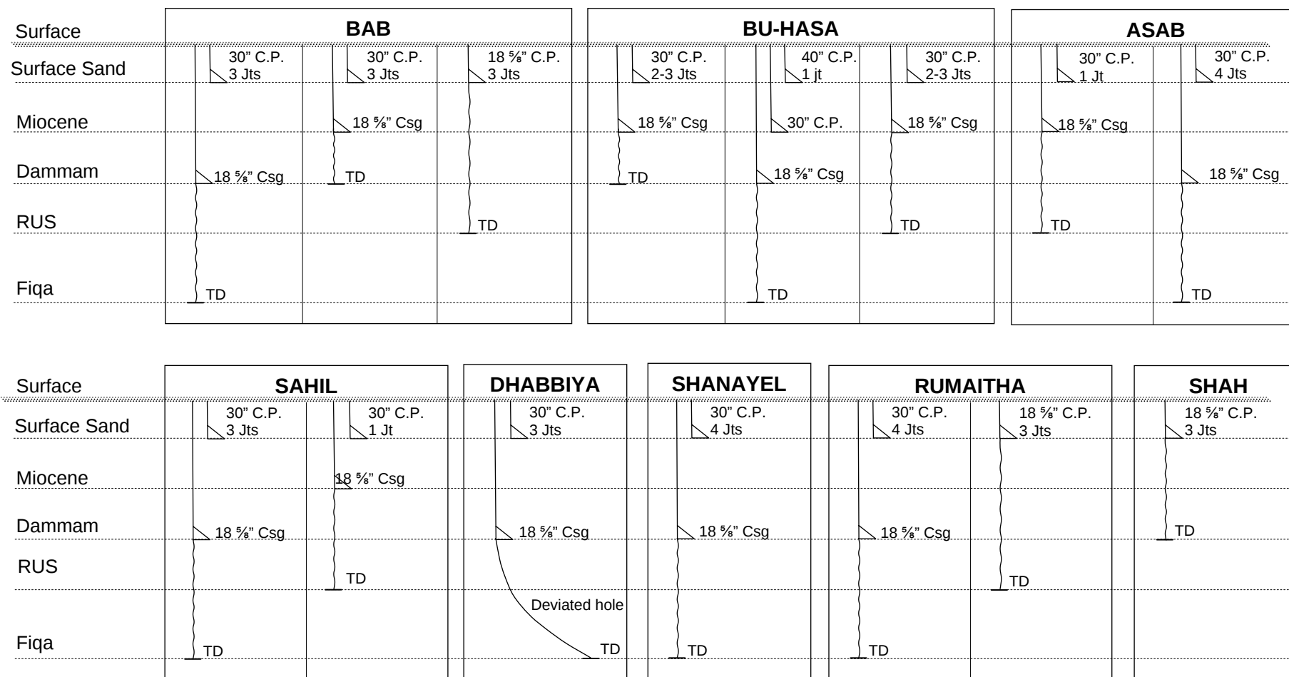
Figure 2- 22: : – ADCO's Typical 17 1/2" Phase
