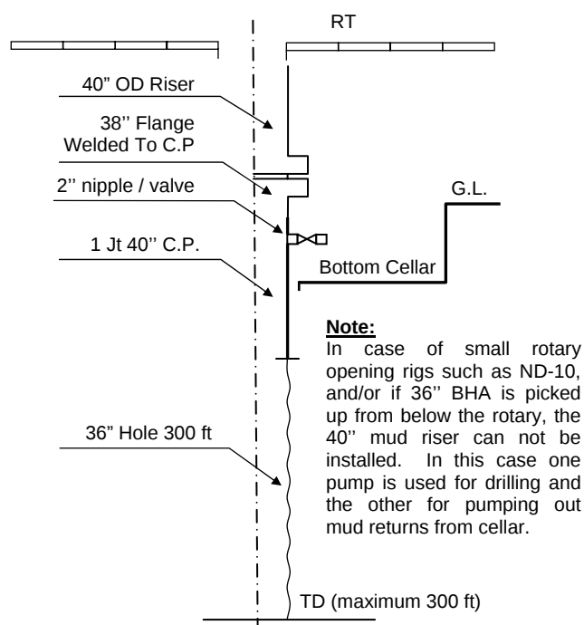
Figure 2-4: Drilling 36" Hole through 40" Riser
