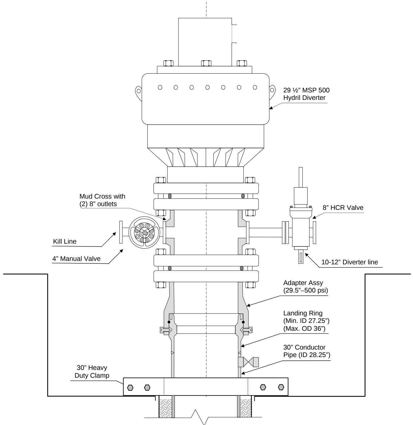
Figure 2-13: Diverter stack for drilling 26" hole
