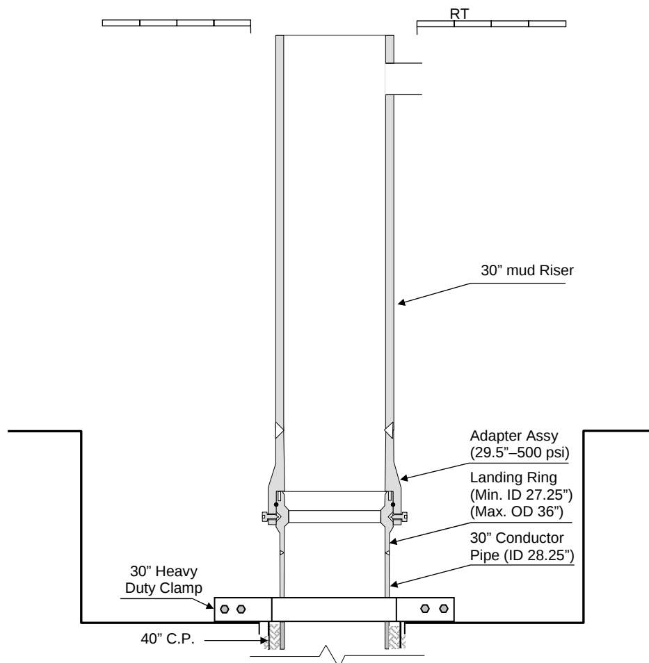
Figure 2-12: 30" Riser for drilling 26" hole
