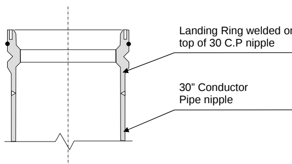
Figure 2-6: landing ring welded to the conductor pipe nipple
