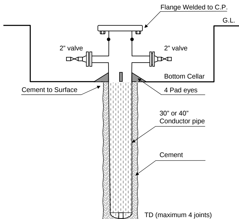
Figure 2-3: Conductor pipe with wellhead
