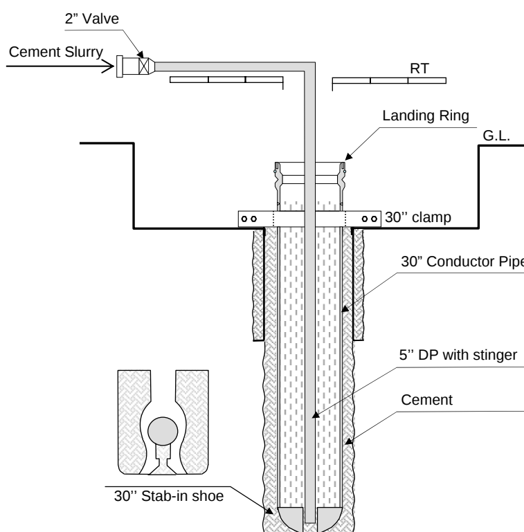
Figure 2-8: Cementing 30" Conductor Pipe with cementing stinger
