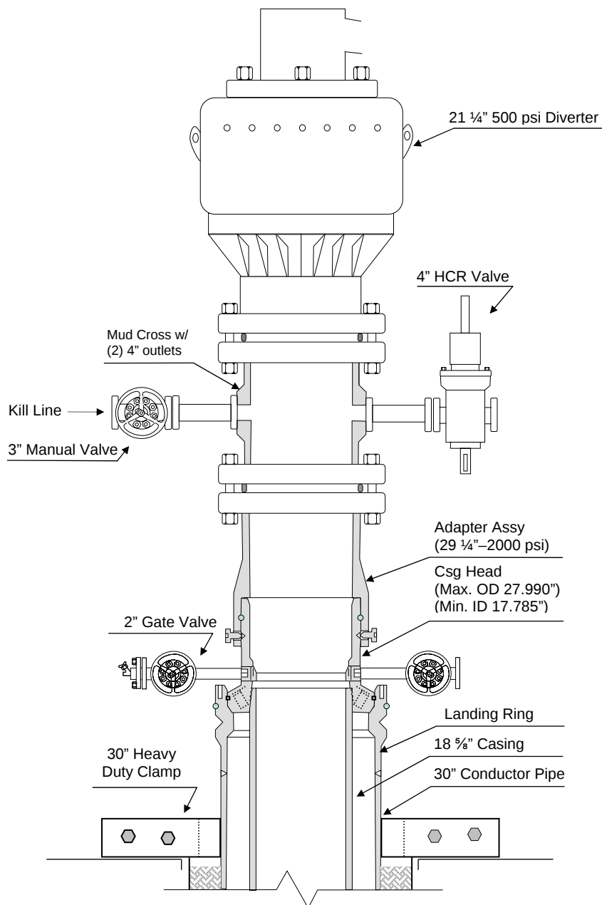
Figure 2- 20: Diverter Stack for Drilling 17.1/2" Hole
