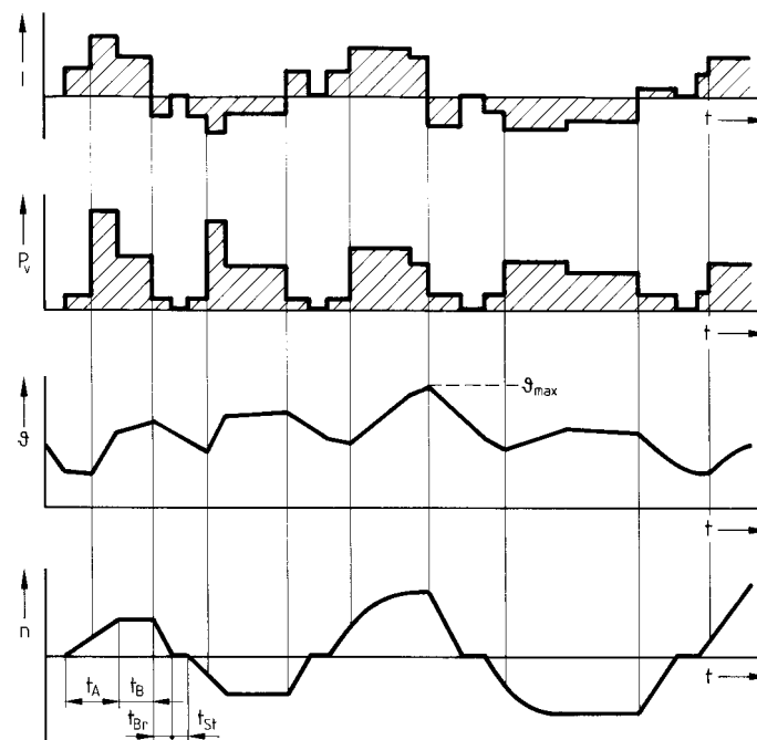
Figure 2.11.1 Duty type S9: Duty with nonperiodic load and speed variations
