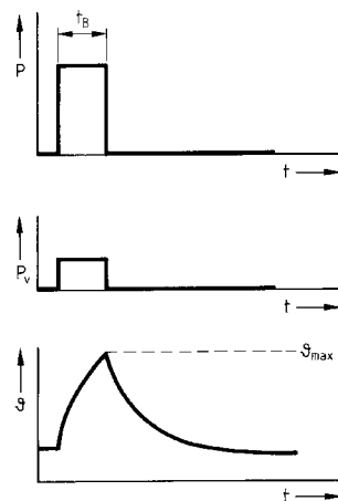
Figure 2.3.1 Duty type S2: Temporary duty
