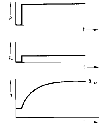
Figure 2.2.1 Duty type S1: Continuous duty
