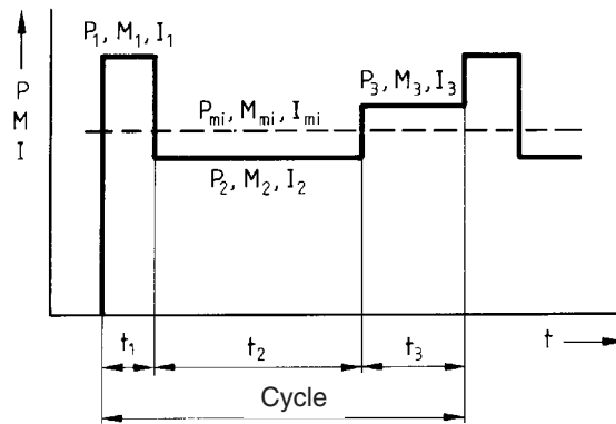
Figure 1.12.1 Determining mean power P_{mi} , mean torque M_{mi} and mean current I_{mi} ( I_{eff} ).
