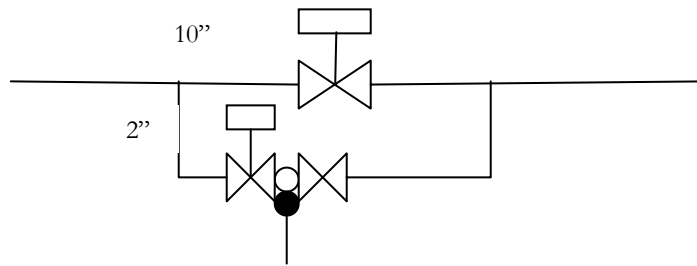
Figure 2: ESD valve Bypass
