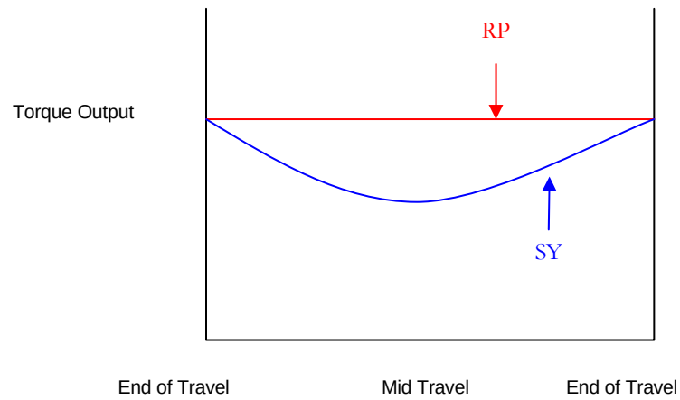
Figure 4: DA actuator torque curve
