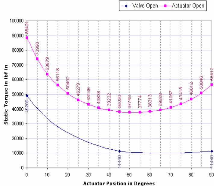
Typical Torque Curve , Source – Bettis
