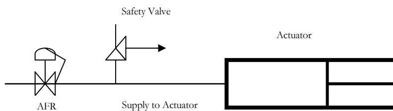
Figure 4: Simplified actuator circuit indicating safety valve
