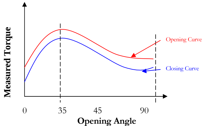
Fig 5: Dynamic Torque Characteristics for Ball valve , Source : Kalsi Engineering Inc.
