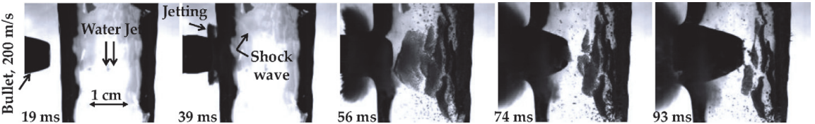
Figure 8. Visualization of a high-speed impact of a 9 mm bullet on a \sim 2 cm water jet. Evidence of secondary cavitation due to shockwaves confinement.
