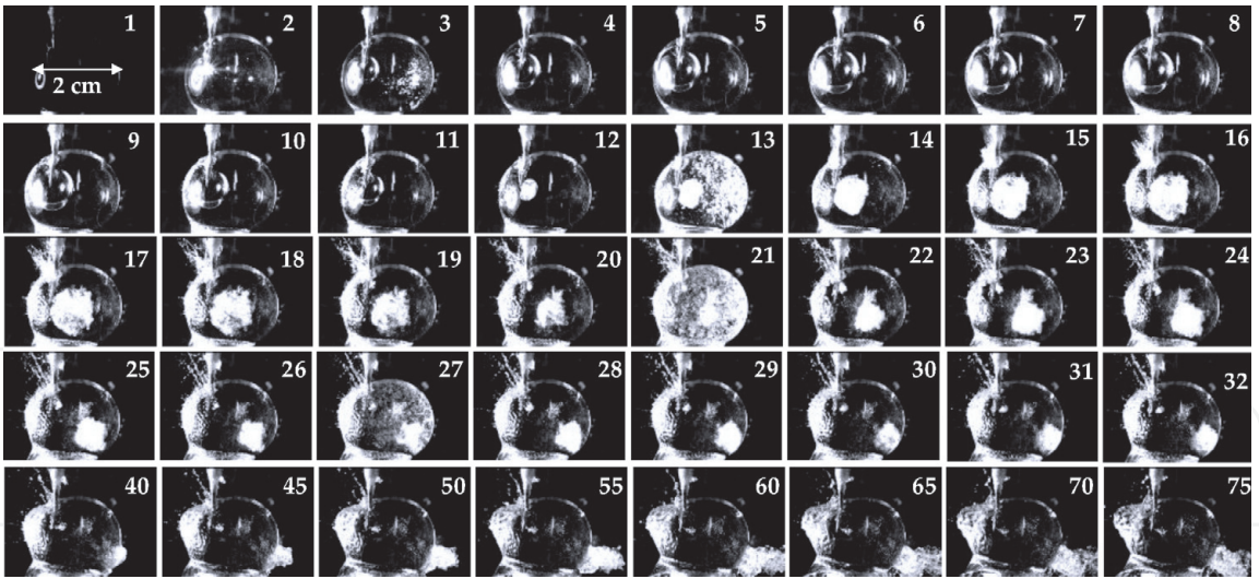
Figure 7. Visualization of a bubble growth and collapse inside a water drop R_{d,min} = 2 cm, R_{b,max} = 1 cm. The inter-frame is 80 \mu s ( 400 \mu s for the last row).
