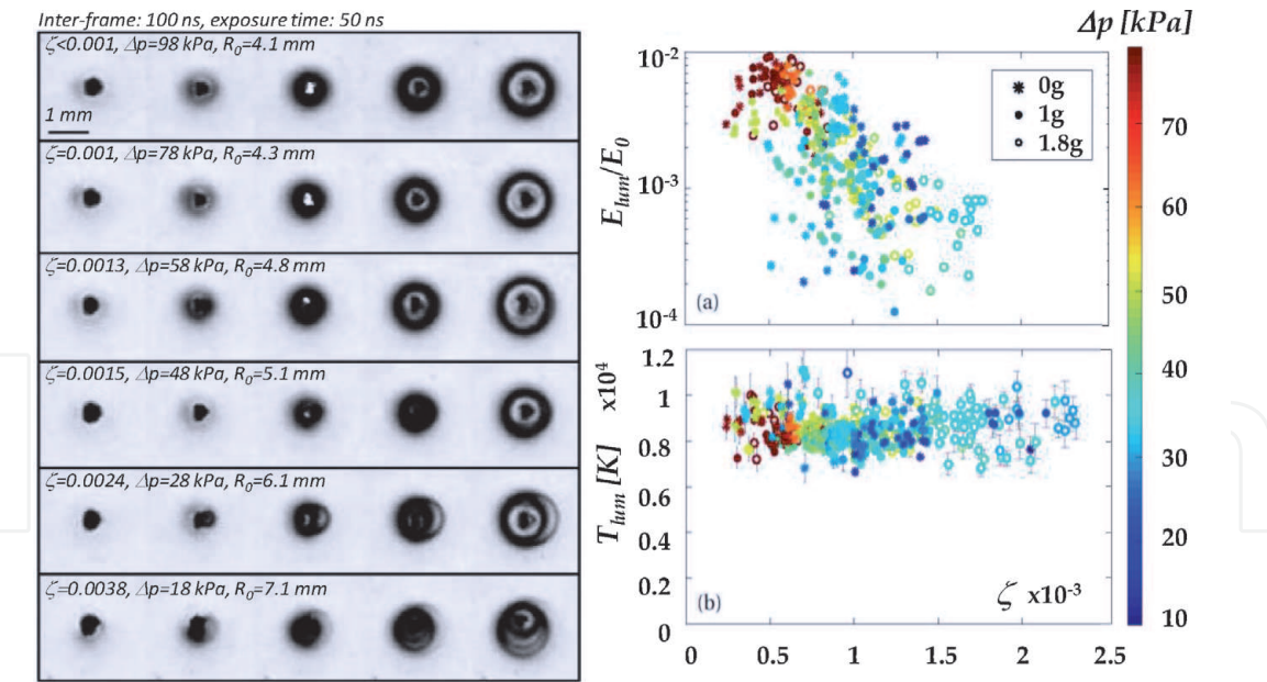
Figure 15. Left: visualization of luminescence emitted by a collapsing bubble, for different values of \zeta . Right: single bubble luminescence (a) relative energy E_{lum}/E_0 and (b) blackbody temperature T_{lum} vs. \zeta . Colors indicate the driving pressures, and symbols indicate the different levels of gravity (adapted from [3]).
