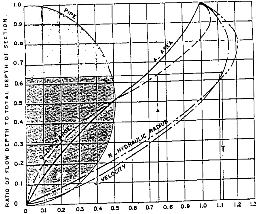
RATIO OF HYDRAULIC ELEMENTS OF THE FILLED SECTION TO THOSE OF THE FULL SECTION.
