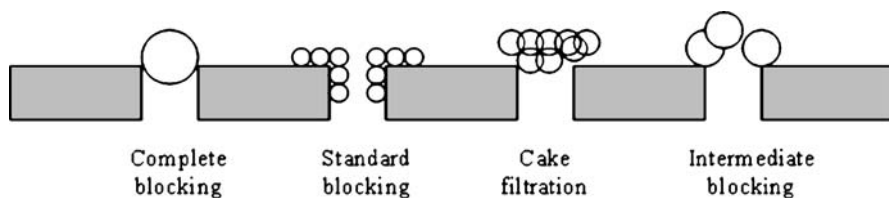
Fig. 9 Fouling mechanisms
