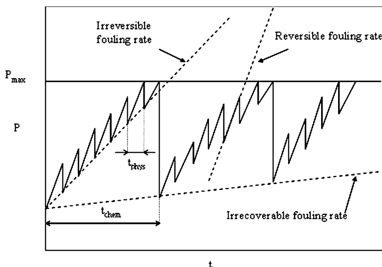
Fig. 10 Fouling rates for different types of fouling ( t_{\text{phys}} – duration of physical cleaning cycle, t_{\text{chem}} – duration of chemical cleaning cycle)
