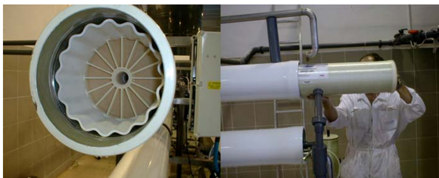
Fig. 6 Connection of the spiral-wound elements
