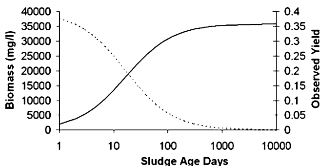
Fig. 11 Net observed yield \cdots and biomass concentration as a function of sludge age in a MBR, HRT=2.7 h, Y=0.4 , k=0.07 \text{ d}^{-1} , k_d=0.06 \text{ d}^{-1} [48]
