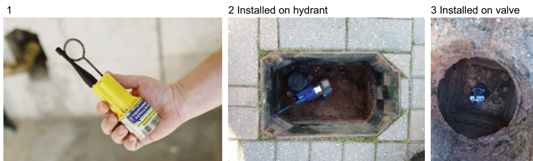
Figure 34 Photographs showing of acoustic loggers (Sources: EPAL (Lisbon) (1), K Atkinson (2, 3)).
