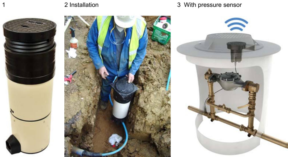
Figure 8 Typical external meter box and Installation (Sources: Plasson (1), J Parker (2), Mueller Water Products Inc. (3)).
