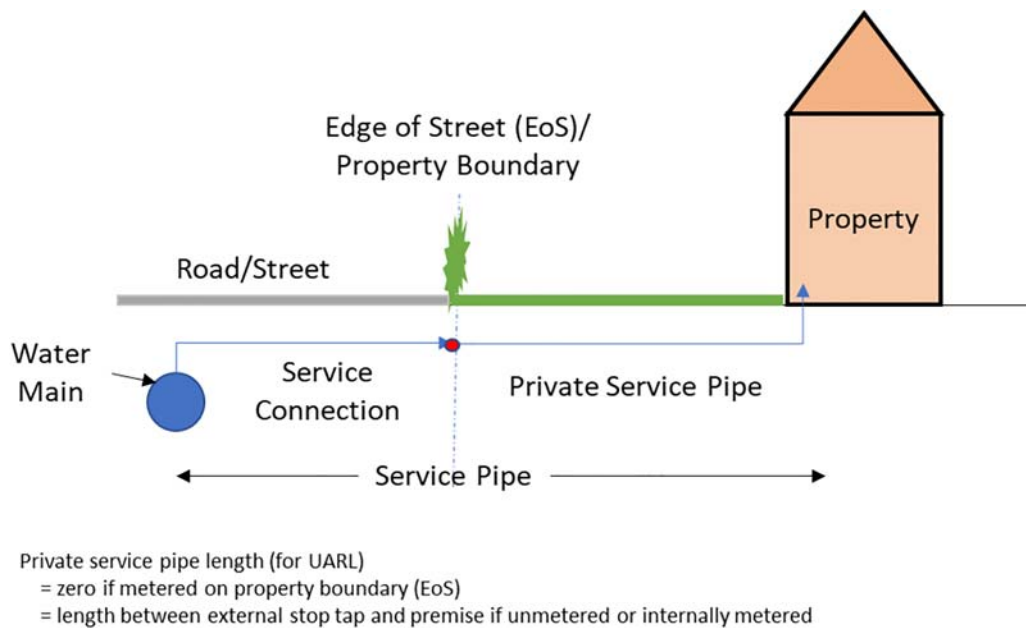
Figure 2 Diagram of a service connection Case 1 (Source: D Pearson).
