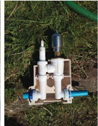
3 Hydrophone on meter box
