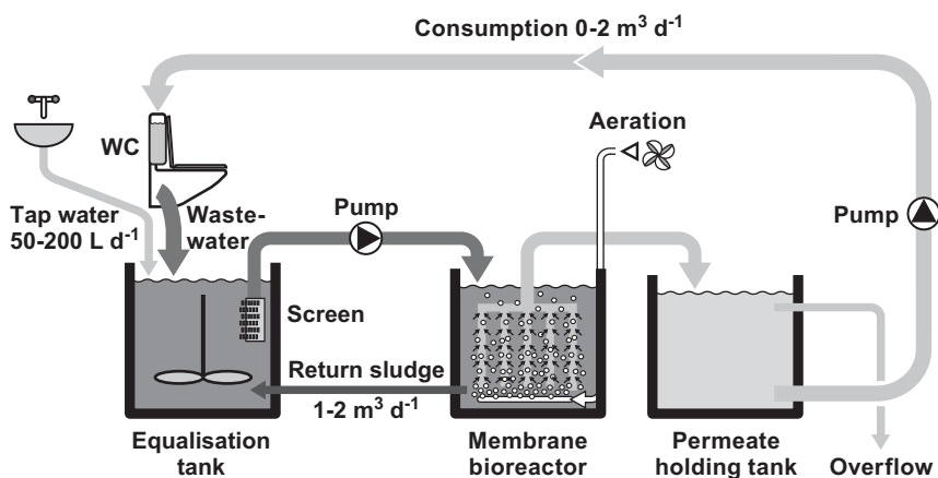
Figure 31.1 Small-scale MBR process scheme for wastewater reuse applied at the Zermatt-Hohtälli cableway station and other on-site treatment projects in Switzerland.
