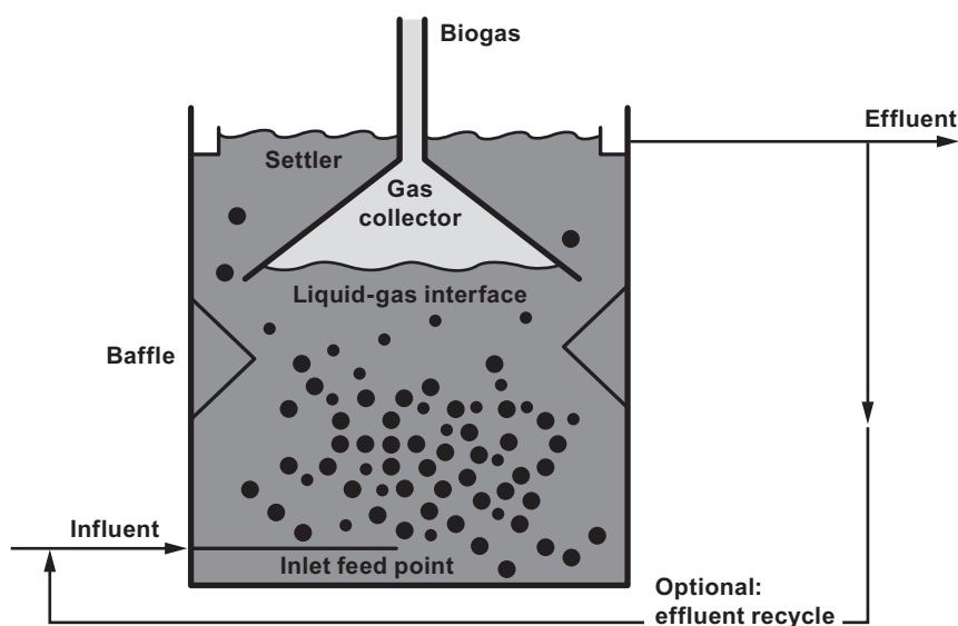
Figure 21.2 Schematic of an upflow anaerobic sludge blanket reactor (UASB).
