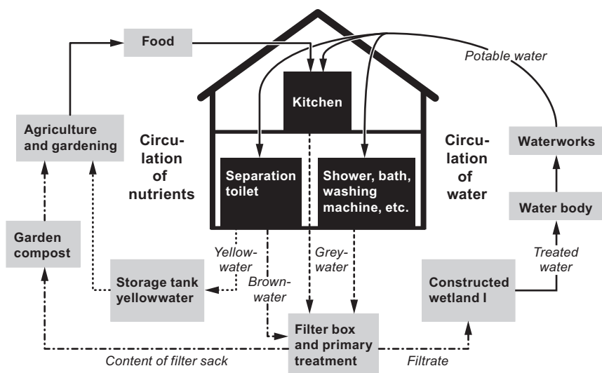
Figure 29.2 Closing the water and nutrient loop in the Lambertsmühle demonstration project (Bastian et al. 2005).
