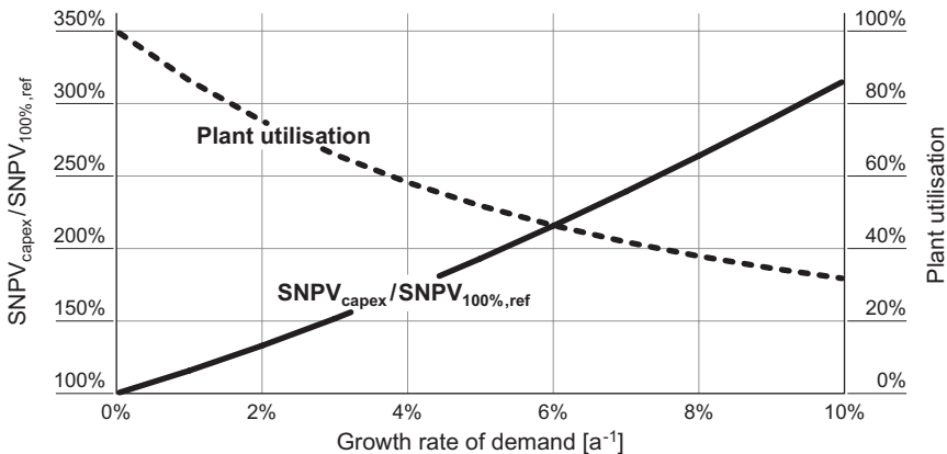
Figure 7.3 The effect of overcapacity on specific investment costs (capex). The solid line shows the increase of specific capital costs ( SNPV_{\text{capex}} ) as a function of the (exponential) growth rate of demand over the assumed lifespan of 30 years. The values are normalized with SNPV_{100\%,\text{ref}} which is equal to the SNPV with no growth (= present value of capex divided by the maximum capacity). No interest rate assumed. The dotted line shows the average plant utilization as a function of growth rate. Adapted from Maurer (2009).
