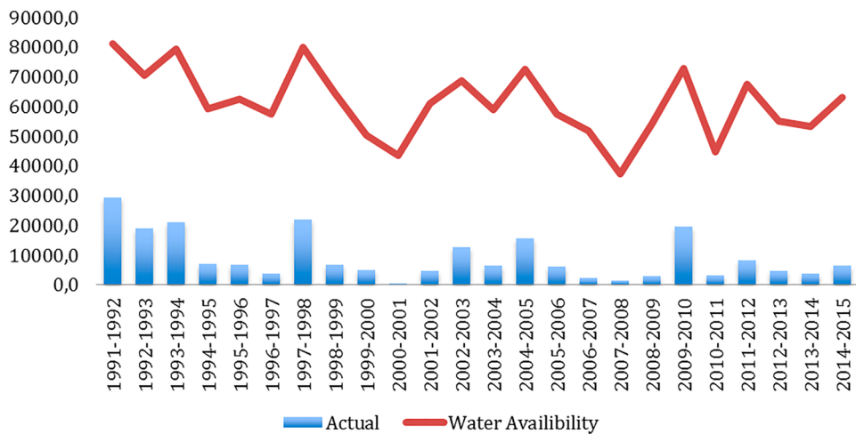
Figure 18.5 Actual water supply to the Amudarya delta, Mm³. Samanbai station, discharge from Suenli and Kyzketken canals and collecting drains.
