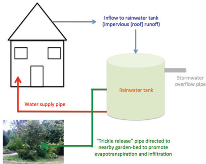
Figure 13.3 An allotment-scale rainwater tank configured with a 'trickle release' pipe.
