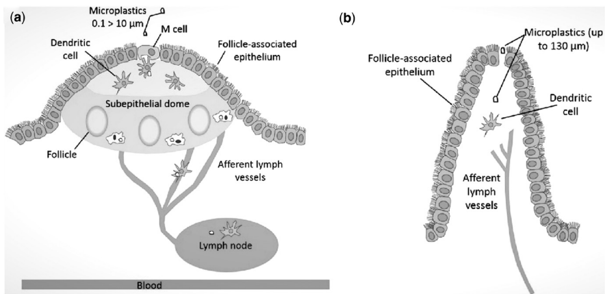
Figure 2.27 Predicted pathways of MP uptake from the GIT. (a) MP (0.1 > 10 μm) uptake from the GIT lumen via endocytosis by the M cells of the Peyer's patches. M cells sample and transport particles from the intestinal lumen to the mucosal lymphoid tissues. (b) MP uptake from the GIT lumen via paracellular perception. Nondegradable particles, such as MPs, may be mechanically kneaded through loose junctions in the single-cell epithelial layer into the tissue below. Dendritic cells can phagocytose such particles, transporting them to the underlying lymphatic vessels and veins. Distribution of secondary tissues, including the liver, muscles and brain, could occur (Source: Wright & Kelly, 2017 ).
