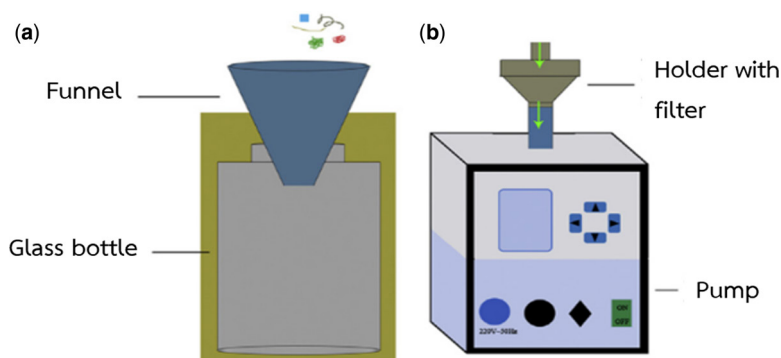
Figure 4.15 Two methods used for atmospheric microplastics sampling. (a) passive atmospheric deposition (b) active pumped samplers (Source: Chen et al. , 2020).
