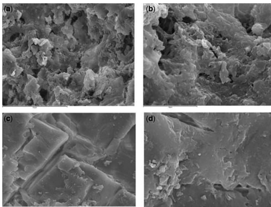
Figure 2.14 The surface topography of eroded plastic pellets from SEM for (a) PE pellets enlarged 1000 times (note the gray scale bar at the bottom of the image; scale bar 60 \mu\text{m} ), (b) PE pellets enlarged 5000 times (scale bar 10 \mu\text{m} ), (c) PP pellets enlarged 1000 times (scale bar 60 \mu\text{m} ), (d) PP pellets enlarged 5000 times (scale bar 10 \mu\text{m} ) (Source: Fotopoulou & Karapanagioti, 2012).
