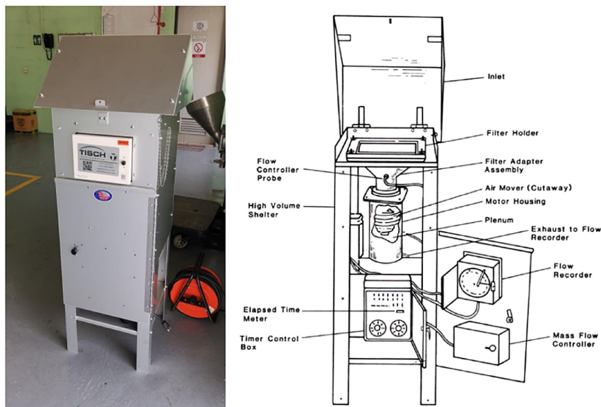
Figure 4.17 High volume sampler used for plastic sampling.
