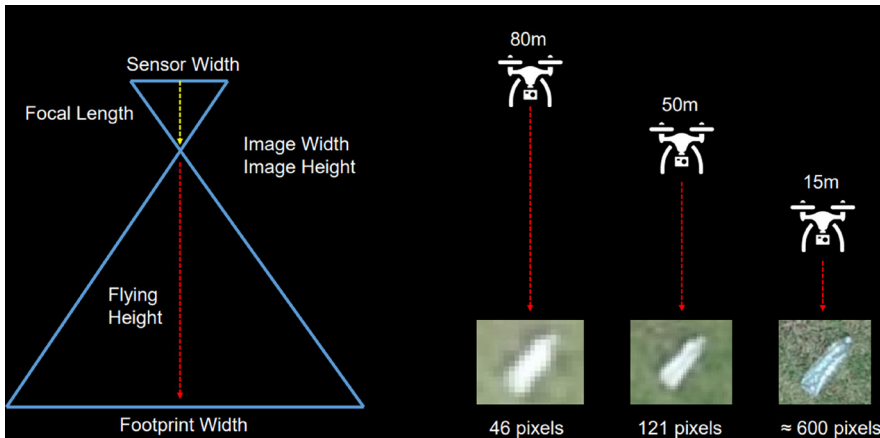
Figure 4.9 Drone image and resolution (Source: Gunasekara, 2019 ).
