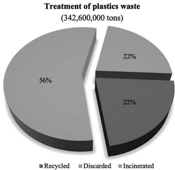
Figure 1.3 Treatment of plastic waste (percentages) (Source: adapted from Geyer et al., 2017 ).
