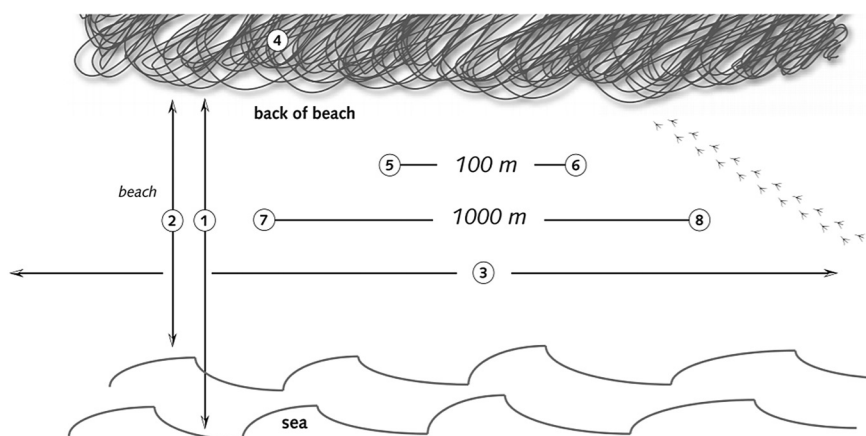
Figure 4.7 OSPAR protocol sampling area of the shoreline monitoring and assessment program (Source: OSPAR, 2010).
