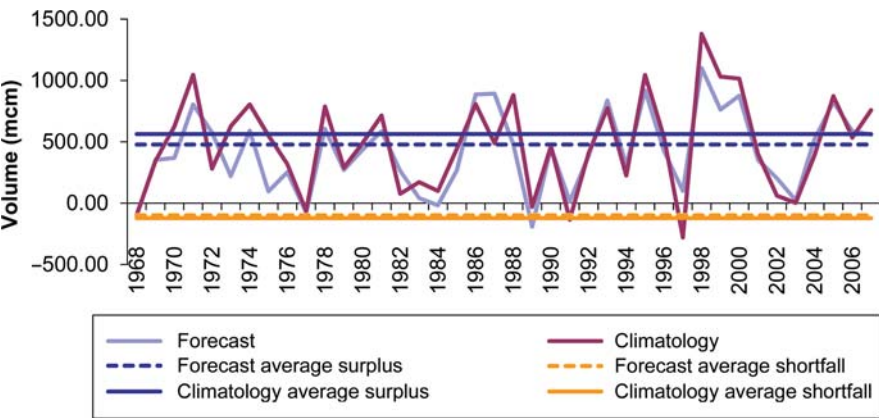
Figure 6.8 Time series of differences between end-of-season reservoir volume and desired minimum threshold (based on the lower rule curve). Please see Table 6.1 for more details. Source: Simulated data from IRI; Angat inflow and storage level data from Philippines National Power Corporation.
