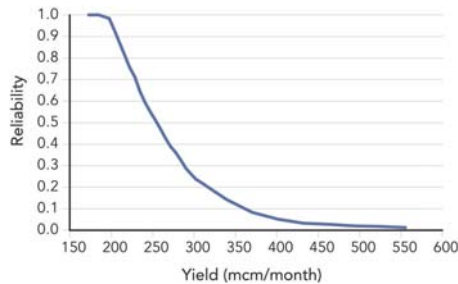
Figure 2.10 Yield-reliability relationship based on the standard operating policy (SOP).
