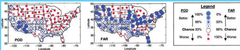
Figure 4.8 Probability of Detection (POD) and False Alarm Rate (FAR) for seasonal precipitation outlooks.
