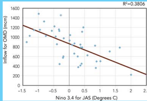
Figure 4.4 Linear regression model between Angat Reservoir inflow during OND and the NINO3.4 index for ENSO during the previous JAS, 1968–2007. Source: SST data from NOAA NCDC ERSST v.2 (Smith & Reynolds, 2004); Angat inflow data from Philippines National Power Corporation.
