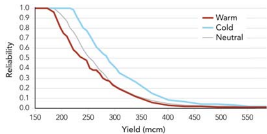
Figure 2.11 Yield-reliability curve conditioned on the Equatorial Pacific SST in July–September.
