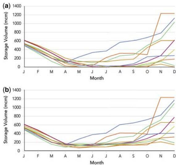
Figure 2.12 Position analysis based on historical inflow traces.
