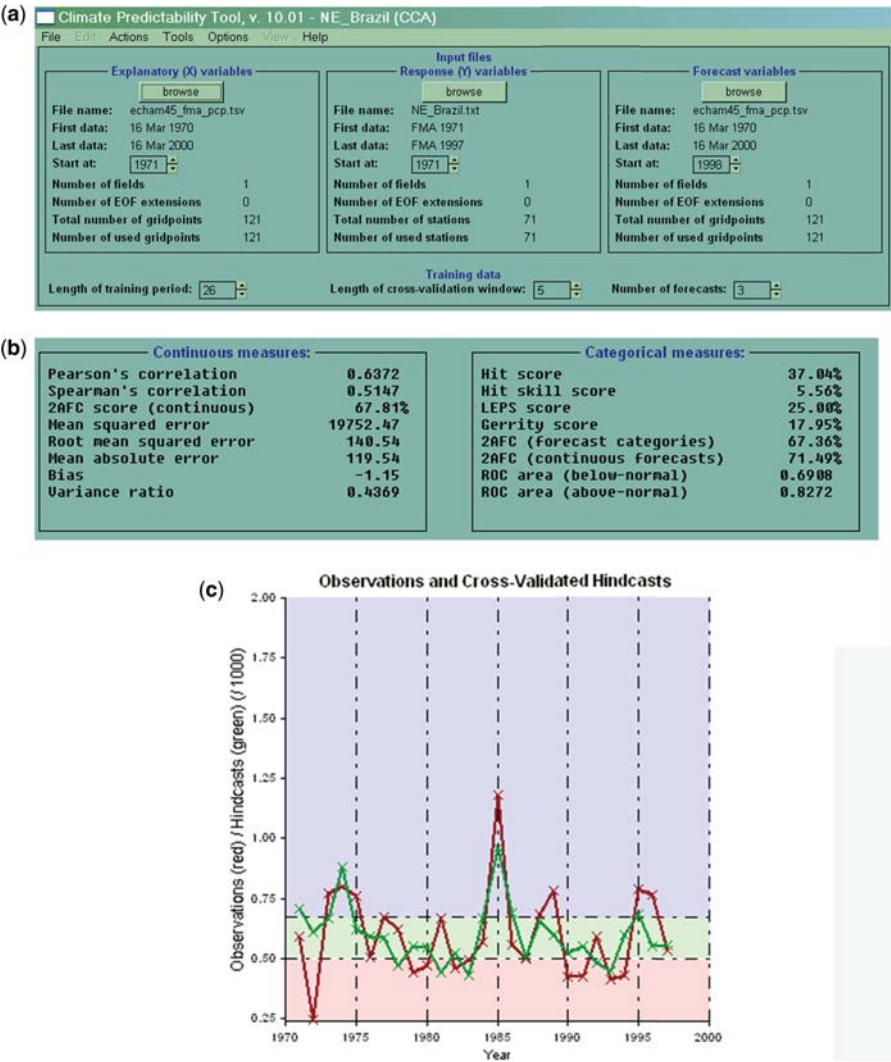
Figure 4.16 Illustration of the application of CPT. Panel (a) shows the model construction; (b) performance statistics; and (c) the performance graph. Panel (a) shows the page in which the user is able to input the datasets and determine the settings to create the desired statistical model; (b) reveals the statistical output from the model, including multiple techniques describing the skill of the statistical model in predicting precipitation based on the SST input; and (c) provides a graph comparing the observation with the cross-validated forecasts overlaid on colors representing the observed climatological tercile categories (purple is above normal, green is near normal and pink is below normal). Source: CPT accessed at http://iri.columbia.edu/climate/tools/cpt .
