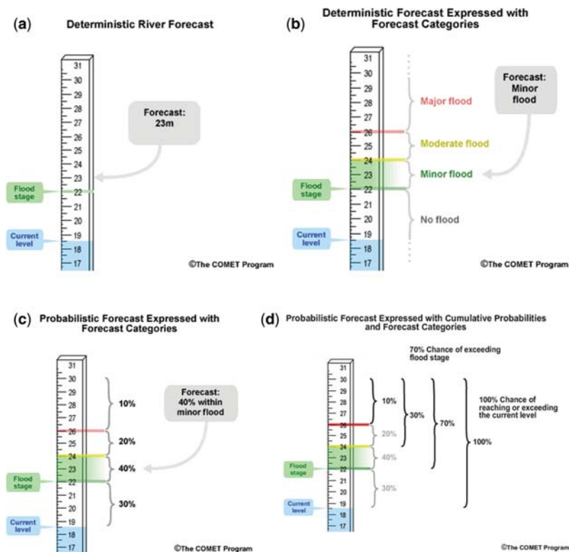
Figure 3.2 Distinguishing between a deterministic and probabilistic forecast. Panel (a) shows an example of a deterministic forecast that predicts a specific inflow level; (b) shows a deterministic forecast that predicts a specific inflow category; (c) shows a probabilistic forecasts that predicts the probability of inflow falling into each category; and (d) shows a probabilistic forecast that predicts the probability of inflow for each category as well as cumulative probabilities across categories of increasing inflow. Source: COMET® Website.
