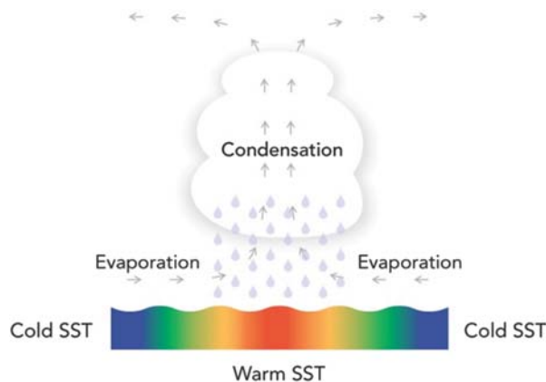
Figure 3.3 A key mechanism for tropical climate on seasonal timescales.
