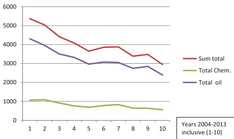
Figure 17.6 Annual numbers of oil and chemical pollution incidents recorded by the Environment Agency (England and Wales, UK) over 10 years, 2004–2013 inclusive (EA, 2015).
