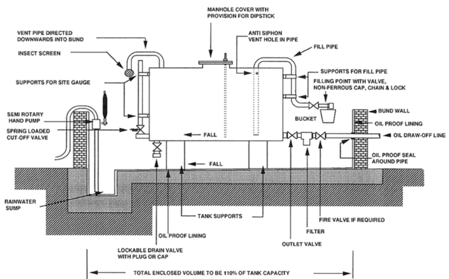
Figure 17.7 Ideally banded oil storage tank (Allcock et al. 1991).
