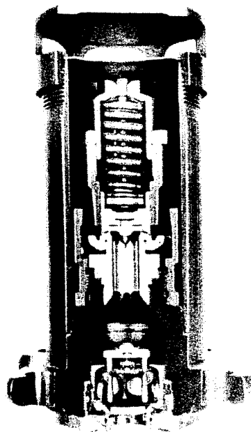
Figure 3.5 Standard Pressure Relief Device
