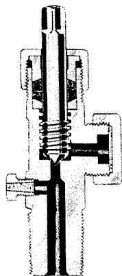
Figure 2.3 Standard Cylinder Valve
