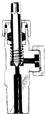
Figure 2.4 Standard Ton Container Valve
