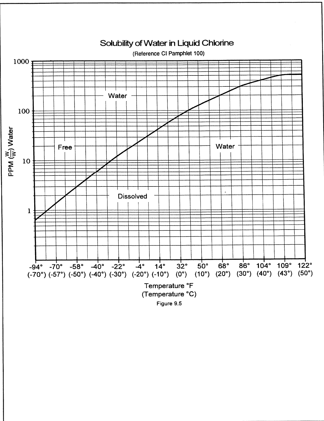
FIGURE 9.5 SOLUBILITY OF WATER IN LIQUID CHLORINE
