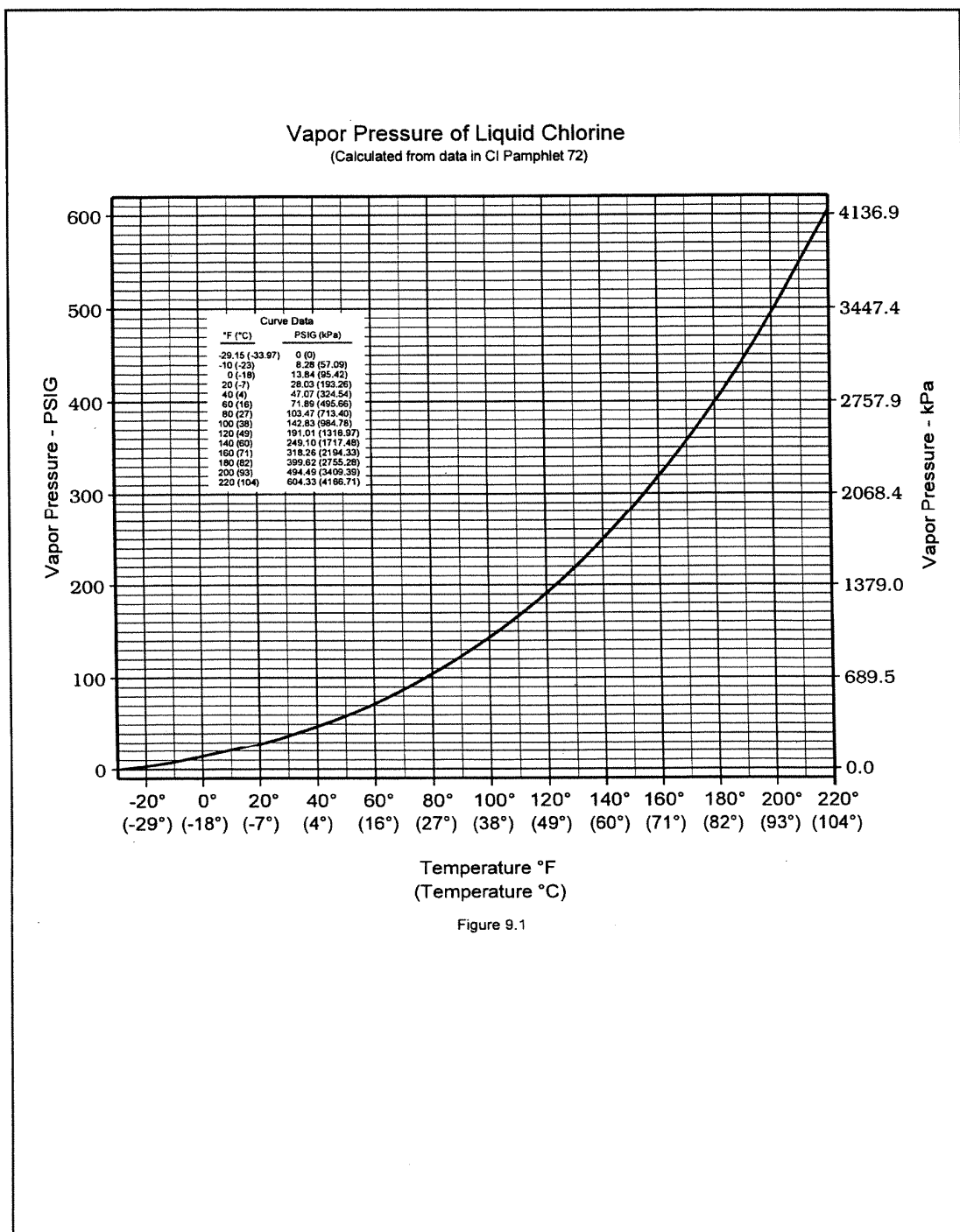
FIGURE 9.1 VAPOR PRESSURE OF LIQUID CHLORINE
