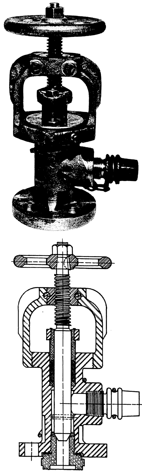
Figure 3.3 Standard Angle Valve
