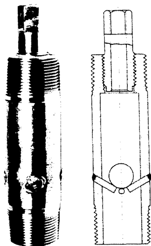
Figure 3.4 Excess-Flow Valve
