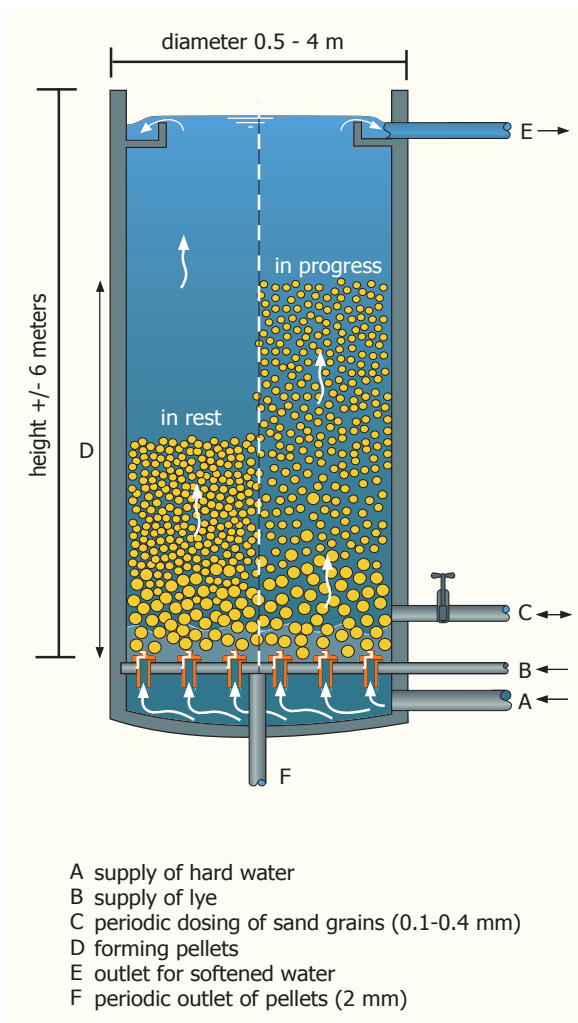
Figure 2 - Schematic representation of a pellet reactor
