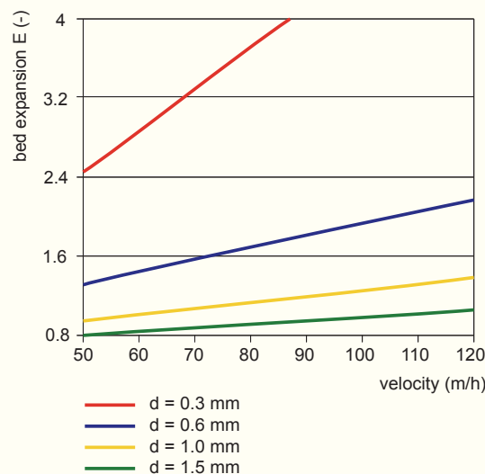
Figure 5 - Bed expansion as a function of pellet diameter and upward velocity
