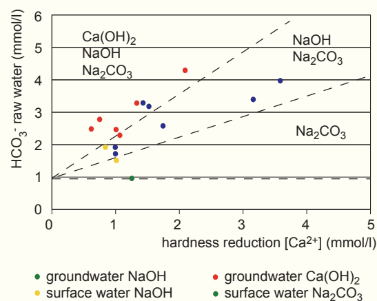
Figure 8 - Application of base as a softening chemical in Dutch practice
