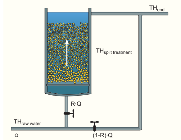
Figure 7 - Principle of split treatment
