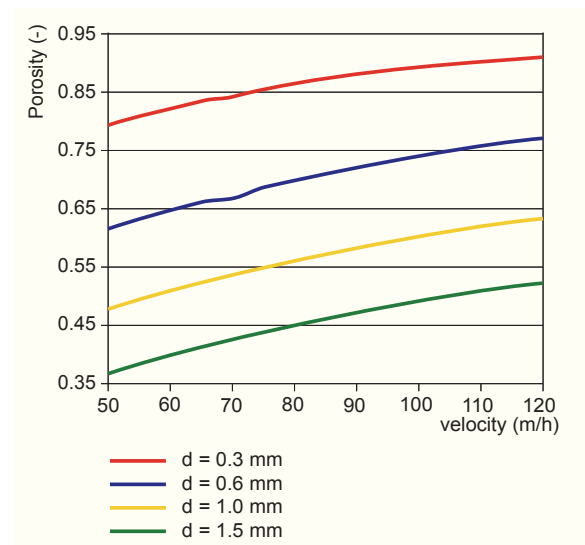
Figure 4 - Porosity as a function of pellet diameter and upward velocity
