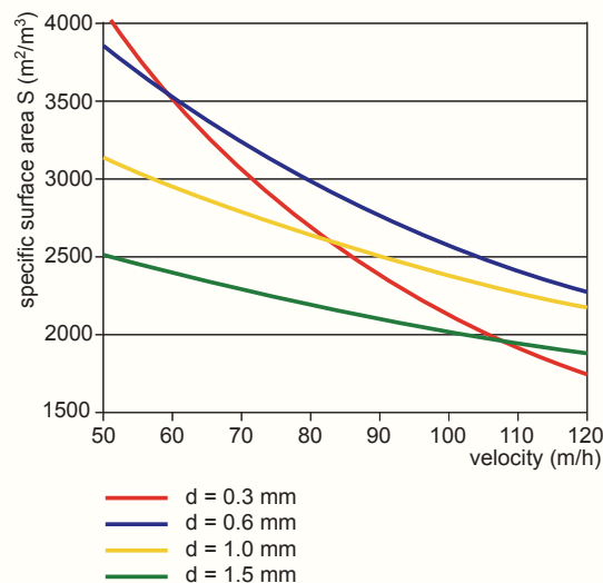
Figure 6 - Specific area as a function of pellet diameter and upward velocity
