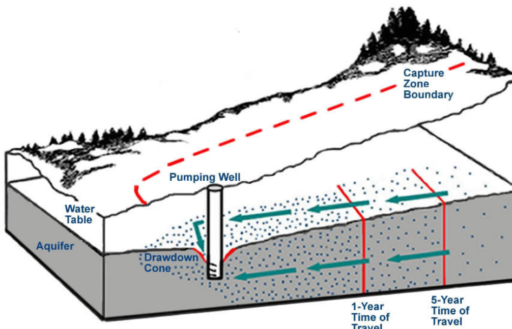
FIGURE 7: EXAMPLE OF CAPTURE ZONE DELINEATION (Well Protection Toolkit, Step 2, MOE)
