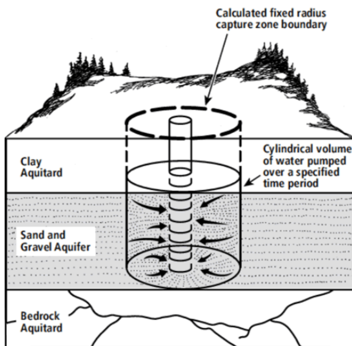
FIGURE 6: EXAMPLE OF CALCULATED FIXED RADIUS (CFR) ( Well Protection Toolkit , Step 2, MOE)
